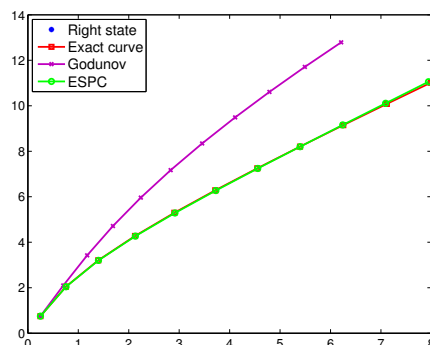
Figure 4.16. Numerical Hugoniot locus for the coupled Burgers equation (4.1) generated by the ESPC and Godunov schemes, compared with the exact Hugoniot locus.
