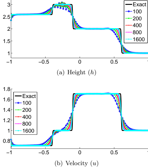
Figure 5.21. Solutions of the linearized shallow water equations (5.8) at time t = 0.25 with initial data (5.12) and boundary data (5.13) computed with the CND scheme at different mesh resolutions. The exact solution is provided for comparison.
