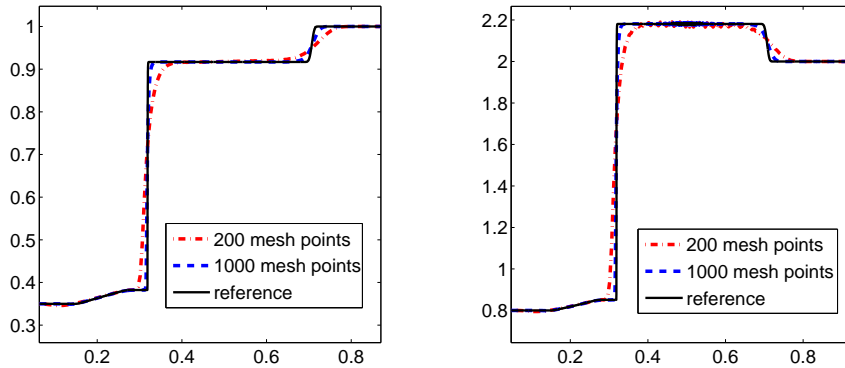
Figure 3.8. Mesh-convergence for the WCD scheme for the dispersive limit of van der Waals fluid with initial data (3.22) with a eighth-order WCD scheme.
