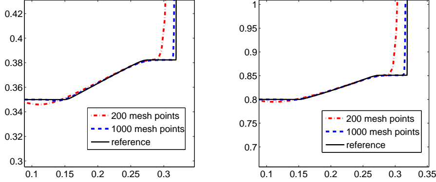
Figure 3.9. Zoom near nonclassical states for the dispersive limit of van der Waals fluid with initial data (3.22) and a eighth-order WCD scheme. Left: Velocity component v . Right: Volume component w .
