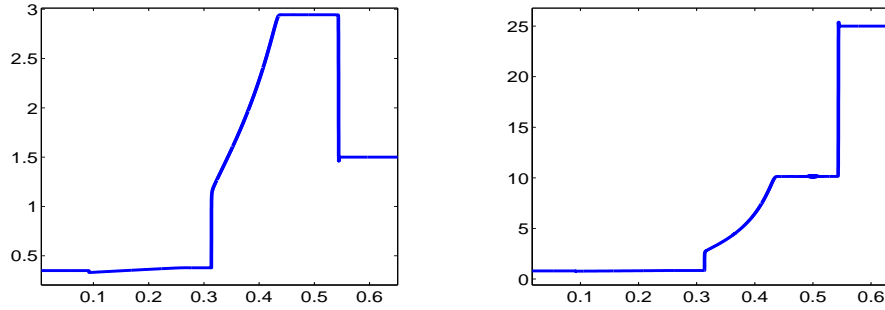
Figure 3.10. Approximation of the Riemann solution with initial data (3.23) resulting in a large jump in volume \tau . Left: Velocity component u . Right: Volume component \tau . Results obtained with an eighth order WCD scheme with 25000 points.
