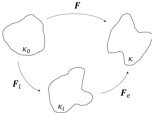
Fig. 14 A decomposition of the deformation gradient tensor \mathbf{F} , where \kappa_0 is the undeformed configuration, \kappa_i is the intermediate configuration and \kappa is the final configuration
