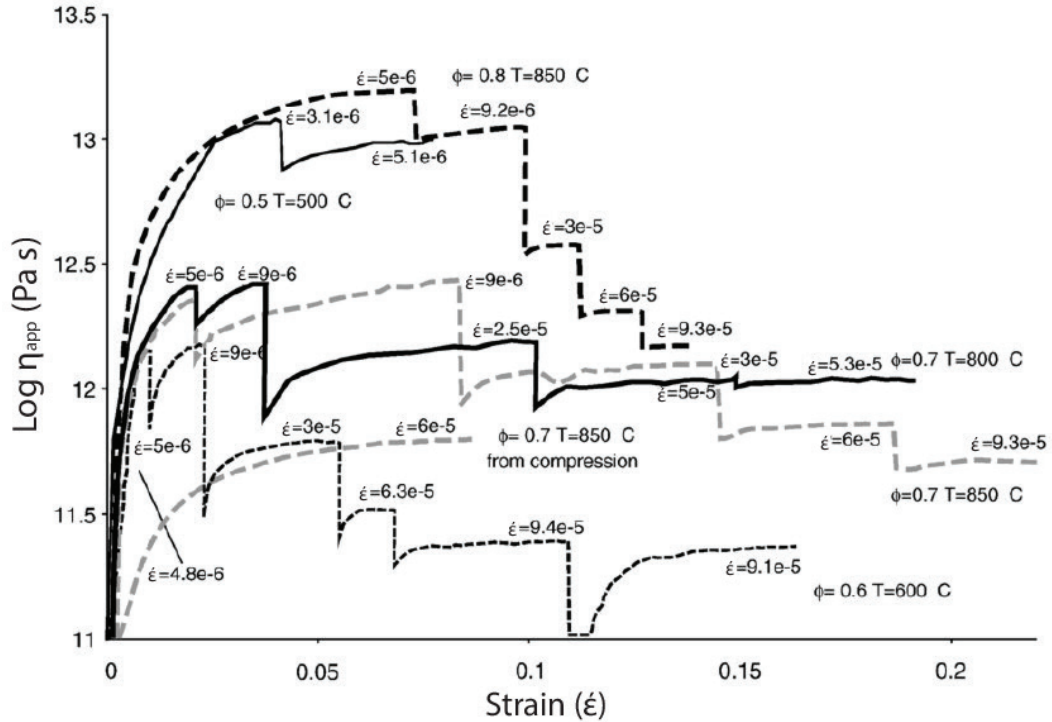
Figure 4.8. Apparent viscosities obtained from individual strain rates ( \eta_{app}=\sigma/\dot{\epsilon} ) plotted versus strain; modified from Caricchi et al. (2007). Increasing the strain rate for any given crystal fraction ( \Phi ) and temperature ( T ) induces a decrease of viscosity, which is interpreted as shear thinning behavior in Caricchi et al. (2007).
