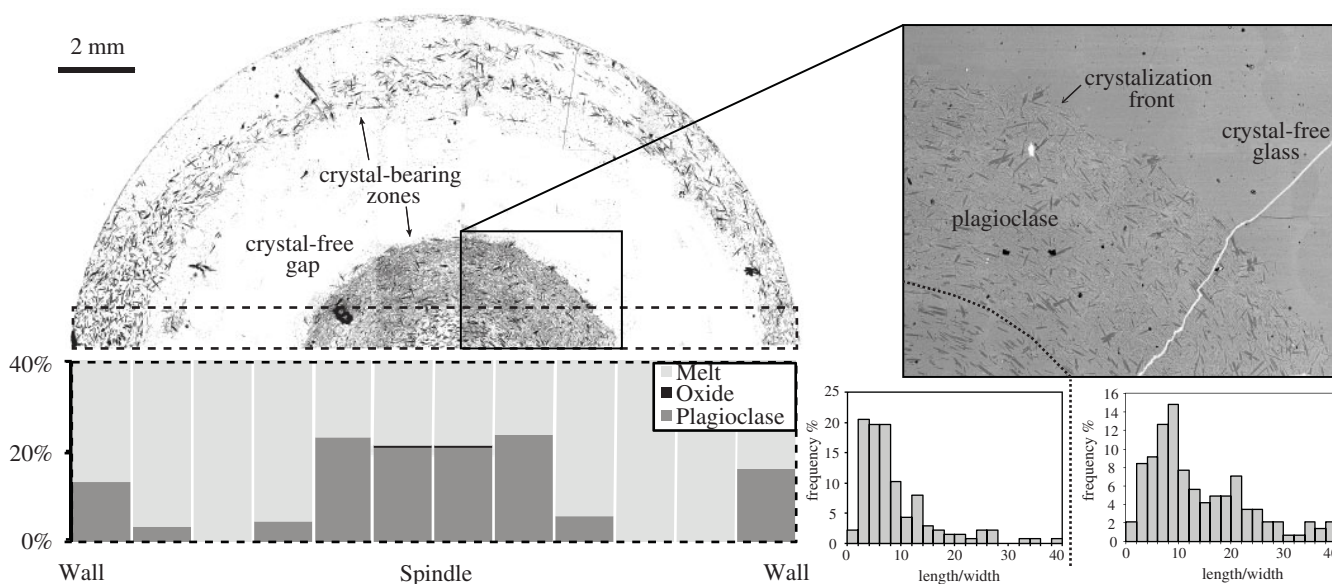
Figure 4. Binary image of the final product quenched during run 2 at 1162°C with the corresponding crystal fraction across the sample (dashed-lined box). The zoomed image is a BSE image showing the crystallization front and two areas within the crystal-bearing zone and corresponding plagioclase aspect-ratio frequency plots.
