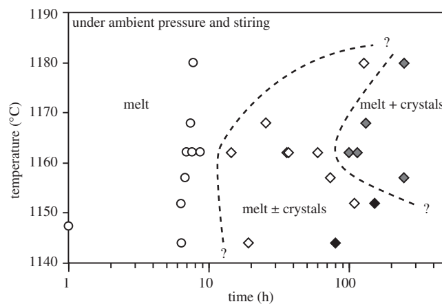
Figure 11. Time-Temperature-Transformation (TTT) diagram built from the kinetic variation of viscosity. Open circles correspond to pure melt phase (at t_1 ), open and black diamonds correspond to the presence of crystals in some amount but not in equilibrium (oxide \pm plagioclase at t_2 and oxide + plagioclase \pm pyroxene at t_3 , respectively) and gray diamonds correspond to the presence of crystals in constant amount (at t_3 ).
