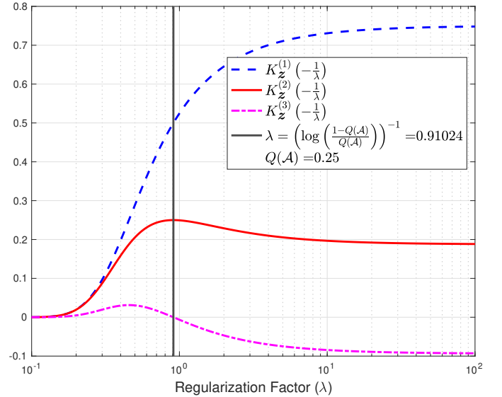
Fig. 3. Mean K_{Q,z}^{(1)}(-\frac{1}{\lambda}) , variance K_{Q,z}^{(2)}(-\frac{1}{\lambda}) , and third central moment K_{Q,z}^{(3)}(-\frac{1}{\lambda}) of the empirical risk in Example 1, with Q(\mathcal{A}) = \frac{1}{4}
