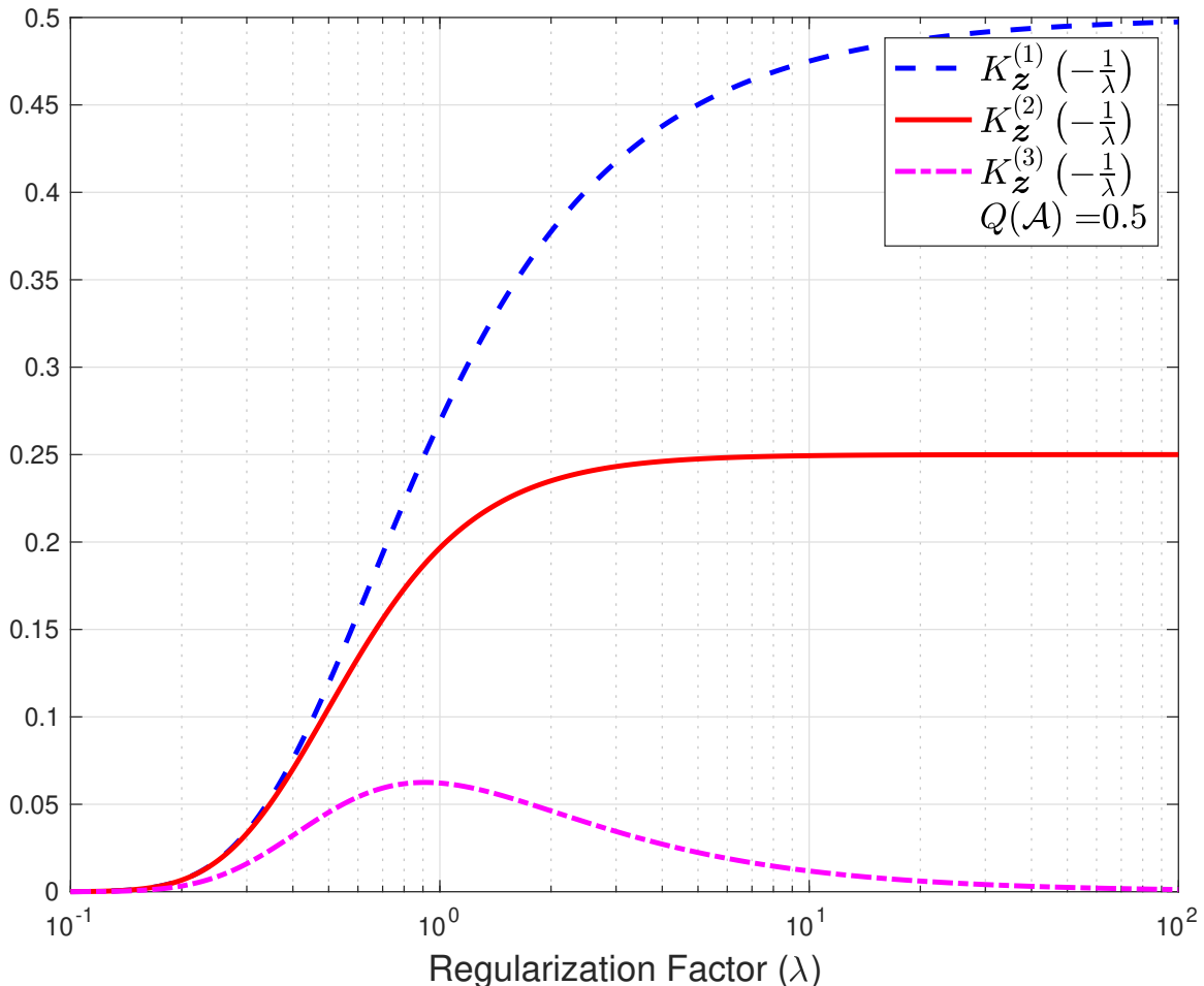
Figure 2: Mean K_{Q,z}^{(1)}\left(-\frac{1}{\lambda}\right) , variance K_{Q,z}^{(2)}\left(-\frac{1}{\lambda}\right) , and third central moment K_{Q,z}^{(3)}\left(-\frac{1}{\lambda}\right) of the empirical risk in Example 1, with Q(\mathcal{A}) = \frac{1}{2}
