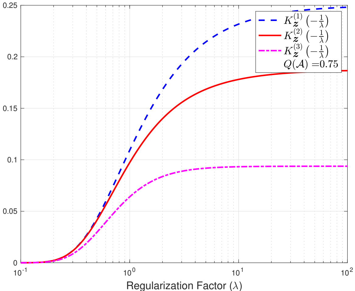
Figure 1: Mean K_{Q,z}^{(1)}(-\frac{1}{\lambda}) , variance K_{Q,z}^{(2)}(-\frac{1}{\lambda}) , and third central moment K_{Q,z}^{(3)}(-\frac{1}{\lambda}) of the empirical risk in Example 1, with Q(\mathcal{A}) = \frac{3}{4}
