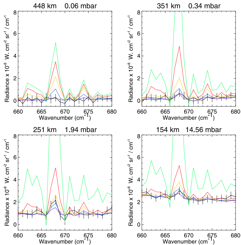
Fig. 24. Same as Fig. 23, except for Cassini CIRS limb spectra from 10^\circ S planetographic latitude in August 2017.
