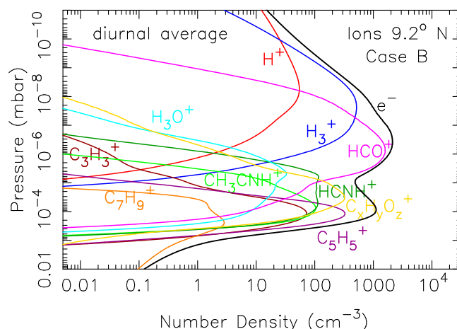
Fig. 8. Ion and electron number densities for our Case B model, assuming diurnally averaged transmission at 9.2^\circ planetocentric latitude. Note that \text{HCO}^+ dominates at the main peak.
