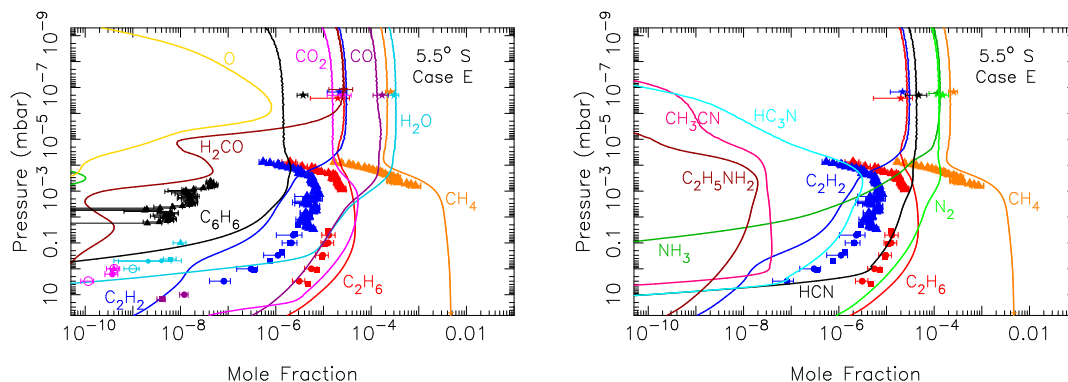
Fig. 11. Mixing-ratio profiles for some neutral hydrocarbons, along with several key oxygen-bearing species (Left) and nitrogen-bearing species (Right) in our Case E model that considers the average orbit 290–292 abundances of incoming species from Serigano et al. (2022). The increase in ring-vapor abundances with decreasing altitude at the top of the model is simply a numerical boundary effect caused by rapid diffusion and the higher-pressure top boundary in this -5.5^\circ latitude model.
