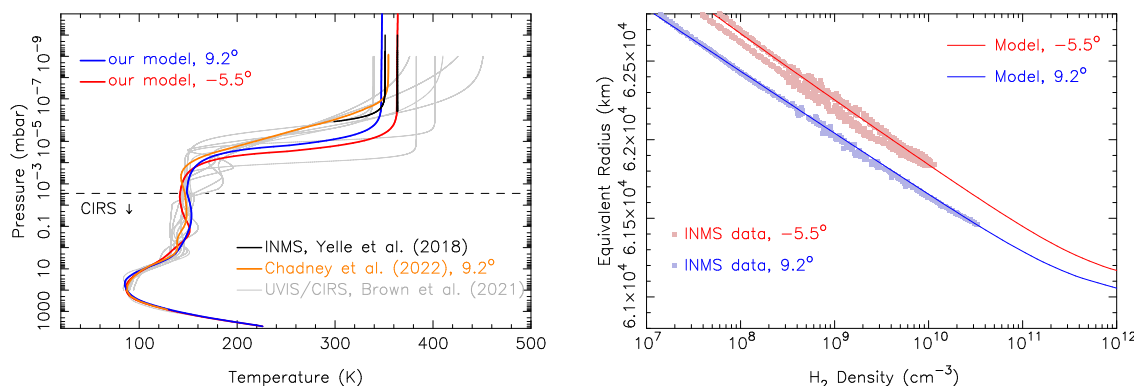
Fig. 1. (Left) Temperature profiles adopted in our model for 9.2° (blue) and -5.5° (red) planetocentric latitude, in comparison with the INMS thermal structure (black) inferred for orbits 293 and 290 by Yelle et al. (2018). The orange curve is the Chadney et al. (2022) 9.2° latitude model, and the gray curves are various low-latitude ( \pm 35^\circ ) temperature profiles derived from a combined analysis of UVIS occultations and CIRS limb retrievals from Brown et al. (2021). Temperatures for our red and blue models at pressures greater than the horizontal dashed line are derived from our combined Cassini CIRS limb and nadir retrievals. (Right) Resulting model H_2 densities at 9.2° (blue) and -5.5° (red) planetocentric latitude, in comparison with INMS-derived H_2 densities (Yelle et al., 2018) as a function of the equivalent radii at 9.2° (gray-blue dots) and -5.5° (gray-red dots) planetocentric latitude. See text for an explanation of equivalent radii. The bifurcation in the measured densities at -5.5° results from differences between the inbound and outbound measurements in orbit 290; the outbound leg has the greater H_2 densities. (For interpretation of the references to color in this figure legend, the reader is referred to the web version of this article.)
