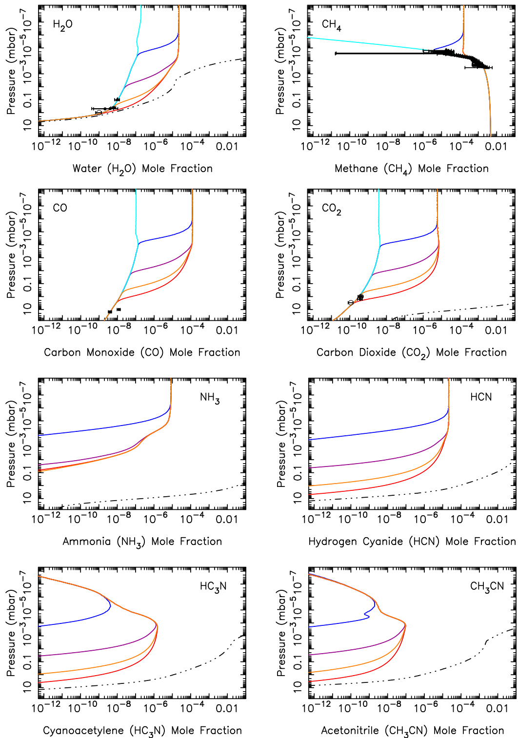
Fig. 15. The mixing-ratio profiles of several species (as labeled) in a time-variable model that starts with the nominal no-ring-influx 9.2^\circ N model results as an initial condition but then adopts a steady Case A ring-vapor flux upper boundary condition starting at time zero. The colored curves show the initial state of the atmosphere (light blue/cyan), and the results after 1 day (darker blue), 4 months (purple), 3 years (orange) and 10 years (red). The ring vapor species flow quickly through the thermosphere and upper stratosphere but more slowly deeper in the stratosphere. The dash-triple-dot lines show the saturation vapor pressure curves for the molecules in question. (For interpretation of the references to color in this figure legend, the reader is referred to the web version of this article.)
