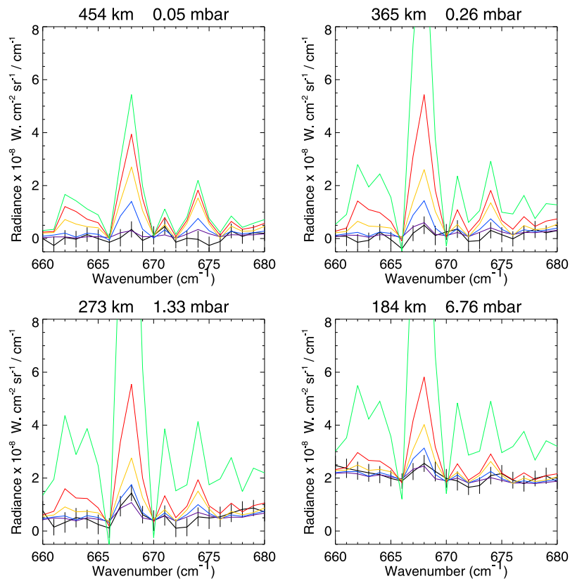
Fig. 23. Cassini CIRS limb spectra showing the detection of CO 2 bands at P \geq 1 mbar from 5^\circ N planetographic latitude in August 2017 (black) at 4 different tangent altitudes, as labeled at the top of each image, compared with synthetic spectra from the nominal 9.2^\circ latitude model (purple), and our time-variable model 4 months (blue), 3 years (orange), 10 years (red), and 100 years (green) after initiating ring-vapor influx at Case A values. (For interpretation of the references to color in this figure legend, the reader is referred to the web version of this article.)
