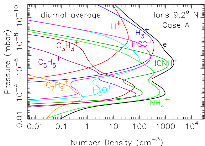
Fig. 6. Ion and electron number densities for our Case A model, assuming diurnally averaged transmission at 9.2° planetocentric latitude. Note the prevalence of nitrogen-bearing ions, in contrast to the nominal model (cf. Fig. 3). The incoming ring vapor significantly changes the ion composition of Saturn's stratosphere compared to the nominal model.
