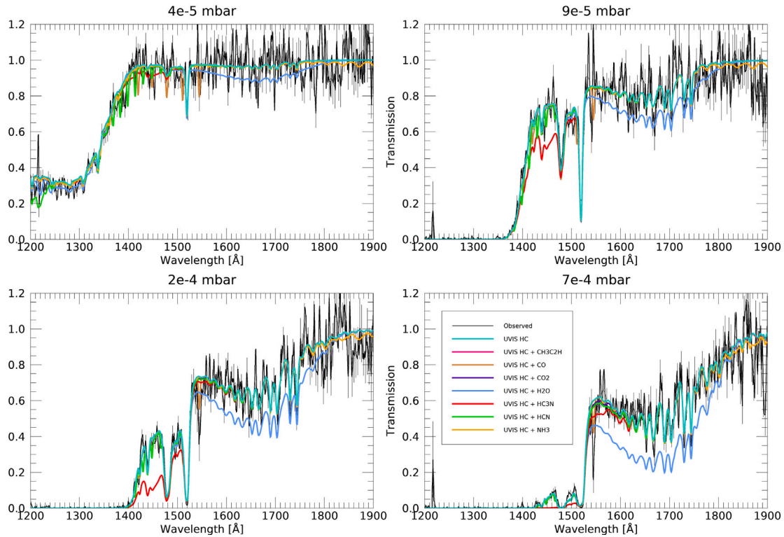
Fig. 25. Line-of-sight transmission of the stellar spectrum through Saturn's atmosphere from the Cassini UVIS \epsilon Ori stellar occultation performed on June 25, 2017 at 12^\circ planetocentric latitude (black curves) compared to the synthetic transmission predicted assuming the retrieved atmospheric vertical profiles of \text{CH}_4 , \text{C}_2\text{H}_2 , \text{C}_2\text{H}_4 , and \text{C}_2\text{H}_6 , along with the retrieved \text{C}_6\text{H}_6 profile at tangent pressures P > 1.38 \times 10^{-4} mbar — where collectively these hydrocarbons are called “HC” in the legend — along with the addition of various ring-derived vapor species from our Case A model (colored lines, as labeled), for tangent radii relevant to P = 4 \times 10^{-5} mbar (Top Left), 9 \times 10^{-5} mbar (Top Right), 2 \times 10^{-4} mbar (Bottom Left), and 7 \times 10^{-4} mbar (Bottom Right). Excess absorption from \text{H}_2\text{O} (blue curves), \text{HC}_3\text{N} (red curves), and to a lesser extent \text{HCN} (green curves) becomes apparent at P \gtrsim 9 \times 10^{-5} mbar, such that the predicted Case A abundances of these species are inconsistent with the UVIS occultation observations. (For interpretation of the references to color in this figure legend, the reader is referred to the web version of this article.)
