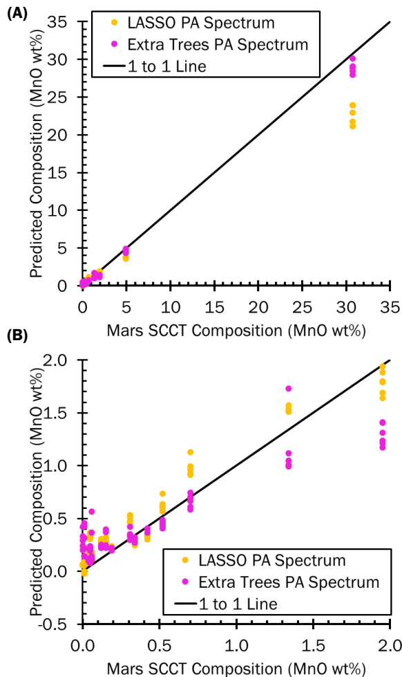
Fig 2: Predictions of SCCTs using LASSO blended submodels and Extra Trees models compared to a 1:1 line for A) the full data range and B) up to 2 wt% MnO.
