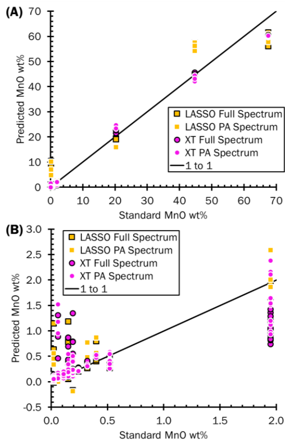
Fig 1: Test Set predictions of the LASSO blended submodels and Extra Trees (XT) models compared to a 1:1 line for A) the full data range and B) up to 2 wt% MnO.
