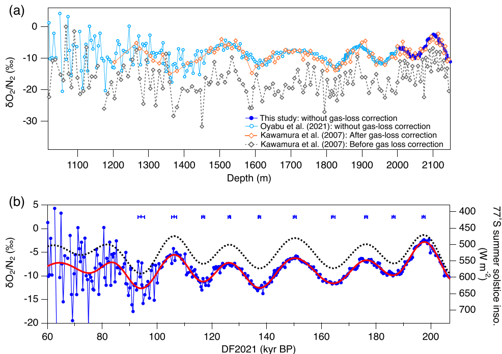
Fig. 3. \delta O_2/N_2 from the DF core. (a) Comparison of the new \delta O_2/N_2 data used for the DF2021 chronology (Oyabu et al., 2021 and this study) with the previous data for the DFO-2006 chronology (Kawamura et al., 2007) from the DF core. While the previous data were treated by post-coring gas-loss correction and outlier rejection, the correction was not necessary for the new data because of improved sample treatment and measurement. (b) New \delta O_2/N_2 data (blue circles), low-pass filtered \delta O_2/N_2 record for identifying age markers (red line), summer solstice insolation at 77°S (black dotted line; computed with the Analyseries software, Paillard et al., 1996 with solution of Laskar et al., 2004), and peak ages in the filtered \delta O_2/N_2 with 2\sigma uncertainty used as age markers for DF2021 (blue markers with error bars at the top). (For interpretation of the references to colour in this figure legend, the reader is referred to the Web version of this article.)
