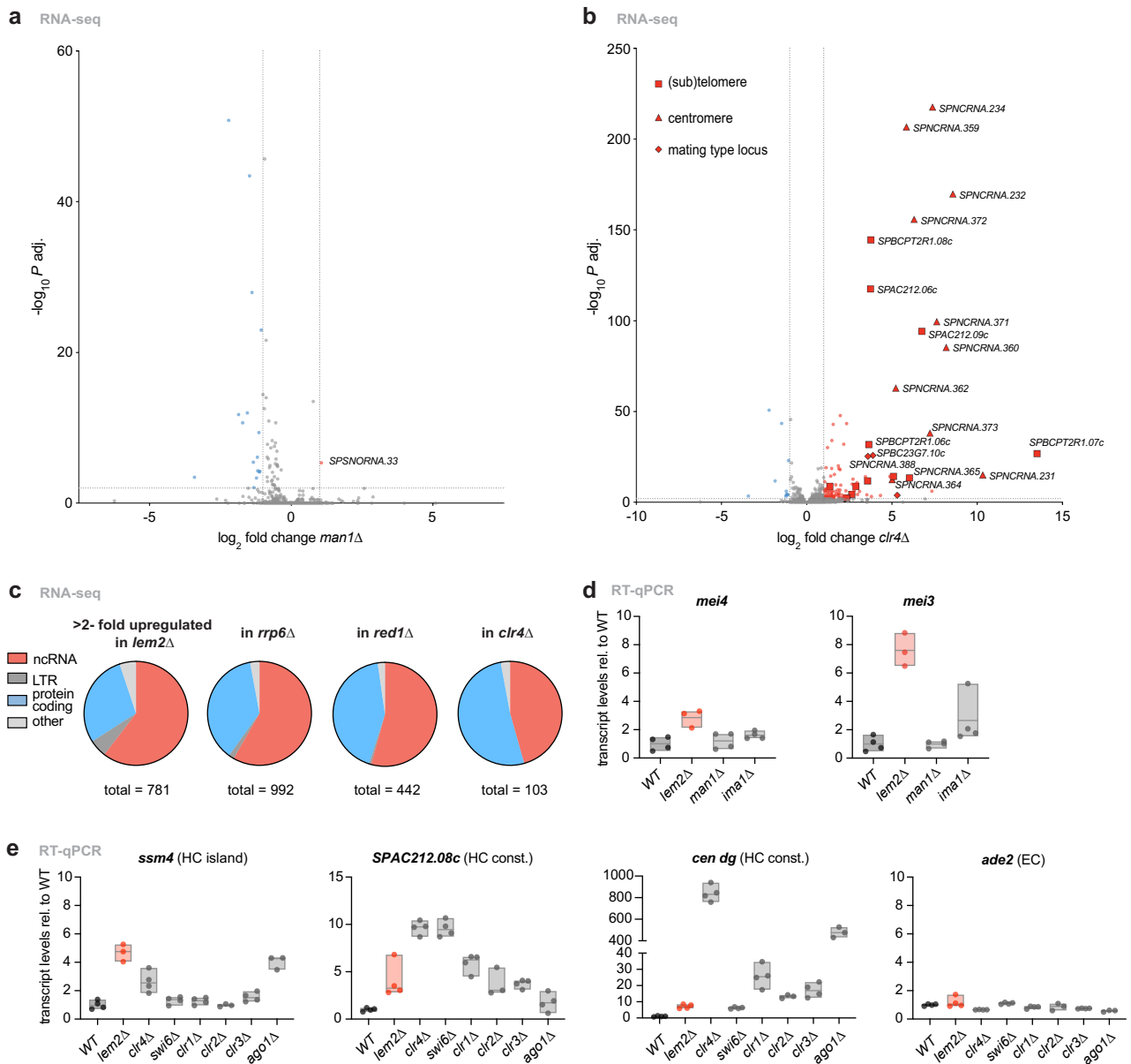
Extended Data Fig. 1 | Lem2 represses non-coding RNAs and meiotic genes. a, b , Volcano plots depicting statistical significance (Y axis) against fold change (X axis) from the RNA-seq data of man1 \Delta vs WT ( a ) and clr4 \Delta vs WT ( b ). Genes significantly up- (red) or downregulated (blue) are highlighted ( \log_2 fold change > 1 or < -1 with P adj. value < 0.01 by the Wald test, as implemented within the DESeq2 framework). c , Pie charts showing of ncRNA, LTR, protein coding, other transcripts (pseudogene, rRNA, snoRNA, snRNA, tRNA). Left: genome-wide distribution of transcript features in a WT genome. Right: transcript feature distribution of the significantly upregulated transcripts in the indicated mutants ( \log_2 fold change > 1 with P adj. value < 0.01 by the Wald test). d , Transcript levels of mei4 and mei3 analyzed by RT-qPCR qPCR ( n = 4 independent biological replicates; except lem2 \Delta : n = 3 ). e , Transcript levels of ssm4 , SPAC212.08c , cen dg , and ade2 analyzed by RT-qPCR ( n = 4 independent biological replicates; except clr2 \Delta , ago1 \Delta : n = 3 ). For ( d , e ), data are normalized to act1 transcript levels or the average of selected euchromatic genes ( act1 + , tef3 + , ade2 + ), respectively, and shown relative to WT. The individual replicates are shown in a floating bar plot and the line depicts the median. HC, heterochromatin; EC, euchromatin.
