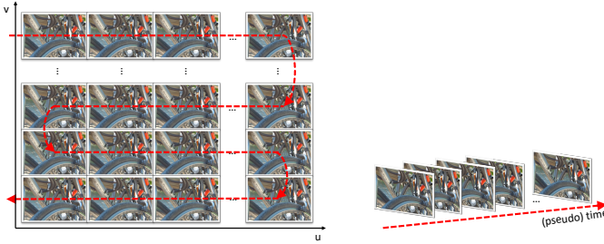
Fig. 2: An example of converting multiview images of a light field into a PVS using the serpentine scan order.
