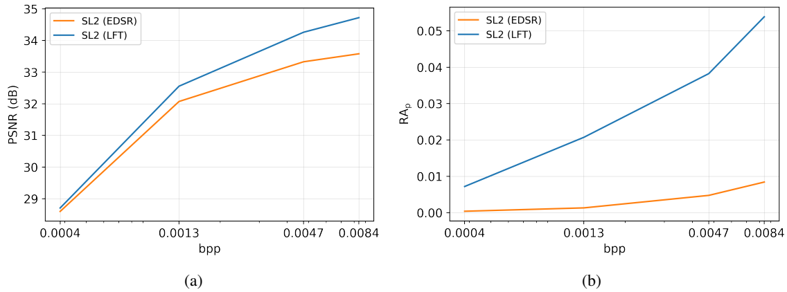
Fig. 17: The comparison between the use of EDSR (SISR) and LFT (LFSR) approaches on the performance of the proposed method in terms of (a) compression efficiency and (b) random access.
