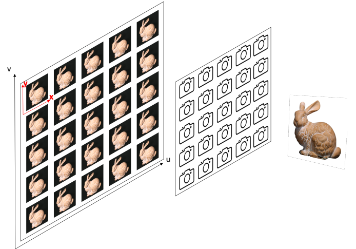
Fig. 1: light fields are typically represented by multiview images. (u,v) represents the view location while (x,y) denotes the pixel location in each view.
