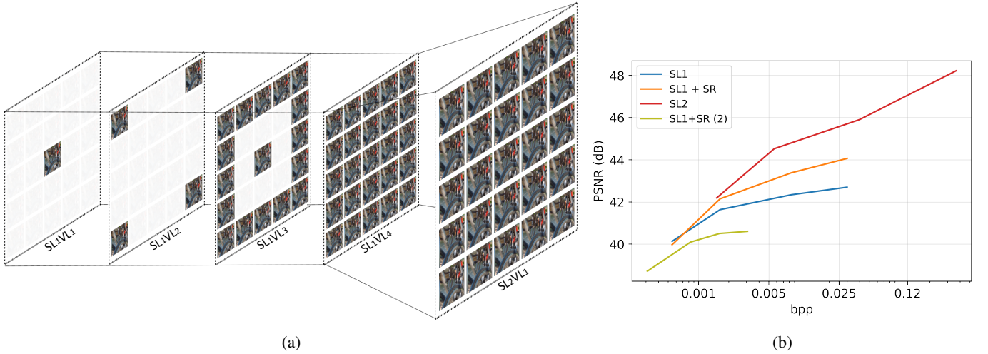
Fig. 16: The corner views in the first spatial layer are used as inputs of RIFE to interpolate all intermediate views between the corner views without adding any quality enhancement layer. In this way, RIFE is run at most thrice to access any arbitrary view in SL_1 . Additionally, DASR is run once to access any arbitrary view in SL_2 without any need to encode/decode any enhancement layer. (a) The example structure for a 5 \times 5 light field. (b) The compression efficiency of the Bunny light field using this structure.
