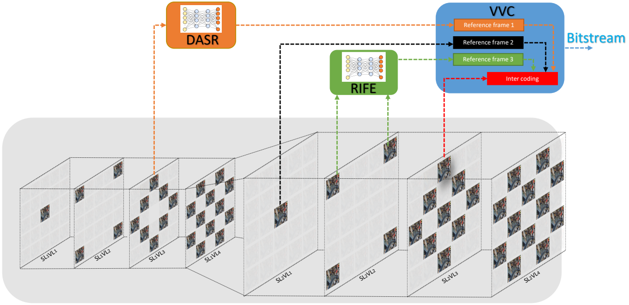
Fig. 7: Encoding workflow for the top view located in SL_2VL_3 .
