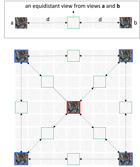
Fig. 5: VL_3 comprises the views that are equidistant from views in VL_1 and VL_2 . \square represents the view of VL_1 , \square represents views of VL_2 , and \square represents views of VL_3 .
