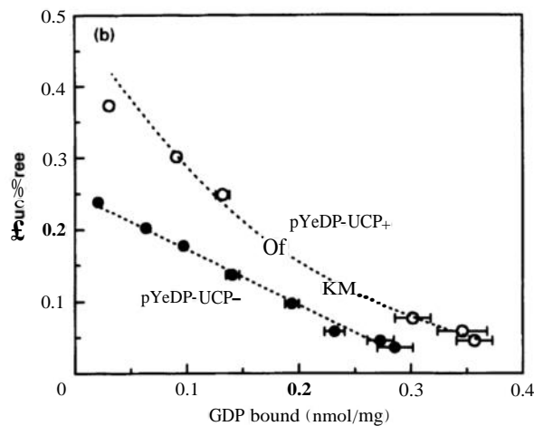
Figure 2 [^3\text{H}]\text{GDP} binding to mitochondria isolated from pYaDP-UCP - and pYeDP-UCP + yeast
