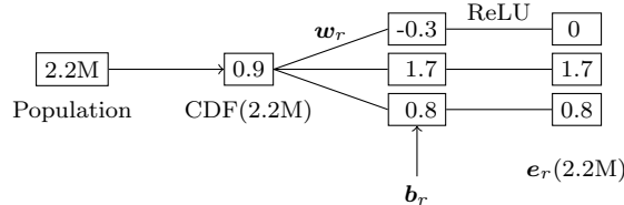
Fig. 6 Embedding numerical values with KEN.
