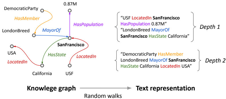
Fig. 3 Graph to text representation in RDF2vec. Random walks are performed on the knowledge graph to generate sentences of tokens. Often, walks are only computed for a subset of entities, here San Francisco. The depth parameter limits the number of hops in the random walk, either forward or backward.
