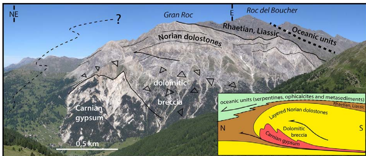
Figure 6: Western slopes of the Gran-Roc massif, a tectonic window cored by a Prepiemont upper Triassic-lowermost Jurassic series and surrounded by oceanic Schistes Lustrés nappes (location fig. 1b). It shows asymmetric anticlinal bending of the upper dolomitic layers, likely associated with a NE-directed ramp over the Carnian evaporites detachment layer. We interpret the interruption of the Prepiemont unit towards the left (NE) as a result of hangingwall cutoff by a D1 NE-directed thrust (cartoon). The eastern side of the massif, behind the crest (visible on fig. 7), is affected by D2 backfolding, producing the rounded shape of this tectonic window.
