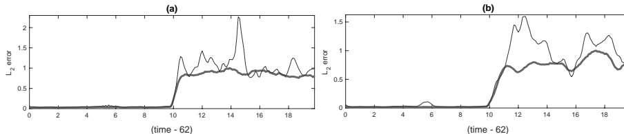
Figure 5: Comparison of the temporal distribution of L_2 spatial errors for case 1C7 (thin line) and 1P4 (thick line) for temperature (a) and v_z vertical flow velocity (b). The curves in each subplot are normalized by the maximum value of the error for case 1P4 (i.e. 20% for temperature and 83% for velocity). The padded approach 1P4 controls errors much better, especially in the second half of the time window.
