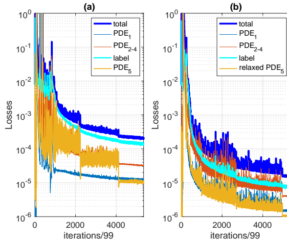
Figure 7: Ra = 2 \cdot 10^9 study: details of the convergence of loss functions for standard PINN 3C1 (a) and best relaxed PINN model (3C1 r , \lambda_5 = 0.1 ) (b) for which the mass conservation PDE constraint (i.e. PDE 5 ) is relaxed during training. PDE 1 : loss term associated with the temperature equation and PDE 2-4 : sum of loss terms associated with the momentum equations, cf. system (3-5).
