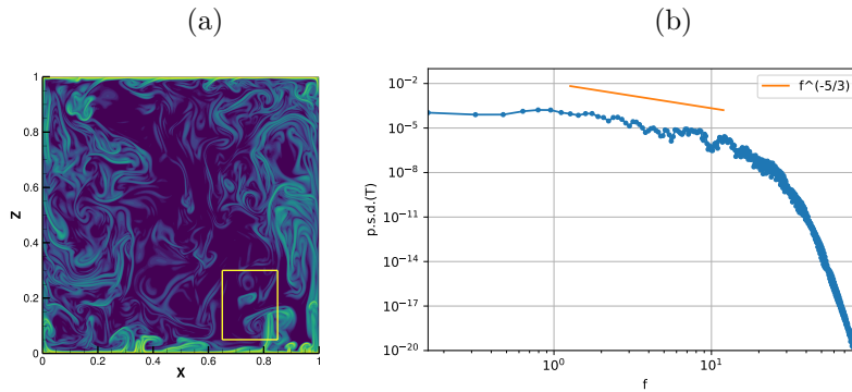
Figure 6: Example of instantaneous heat dissipation isocontours (2D (x, z) slice at (y = 0.25, t = 290.83) ) from DNS of the RB cavity flow at Ra = 2 \cdot 10^9 (a). The domain \Omega_{\text{PINN}} over which the PINN model is trained, is depicted as a transparent box. Temporal power spectrum of temperature at location (x = 0.65, y = 0.25, z = 0.1) (b)
