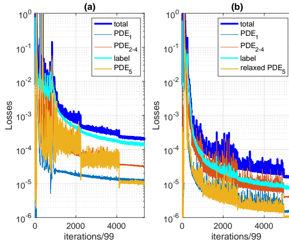
Figure 7: Ra = 2 \cdot 10^9 study: details of the convergence of loss functions for standard PINN 3C1 (a) and best relaxed PINN model (3C1 r , \lambda_5 = 0.1 ) (b) for which the mass conservation PDE constraint (i.e. PDE 5 ) is relaxed during training. PDE 1 : loss term associated with the temperature equation and PDE 2-4 : sum of loss terms associated with the momentum equations, cf. system (3-5).
