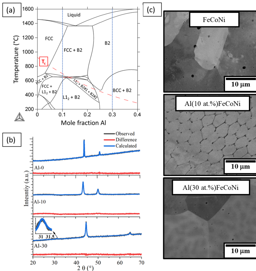
Figure 1. (a) Pseudo-binary isopleth for varying Al in ternary CoFeNi system (b) Rietveld refinement of the X-ray diffraction patterns and (c) SEM backscatter images of Al_x(CoFeNi) CCA.
