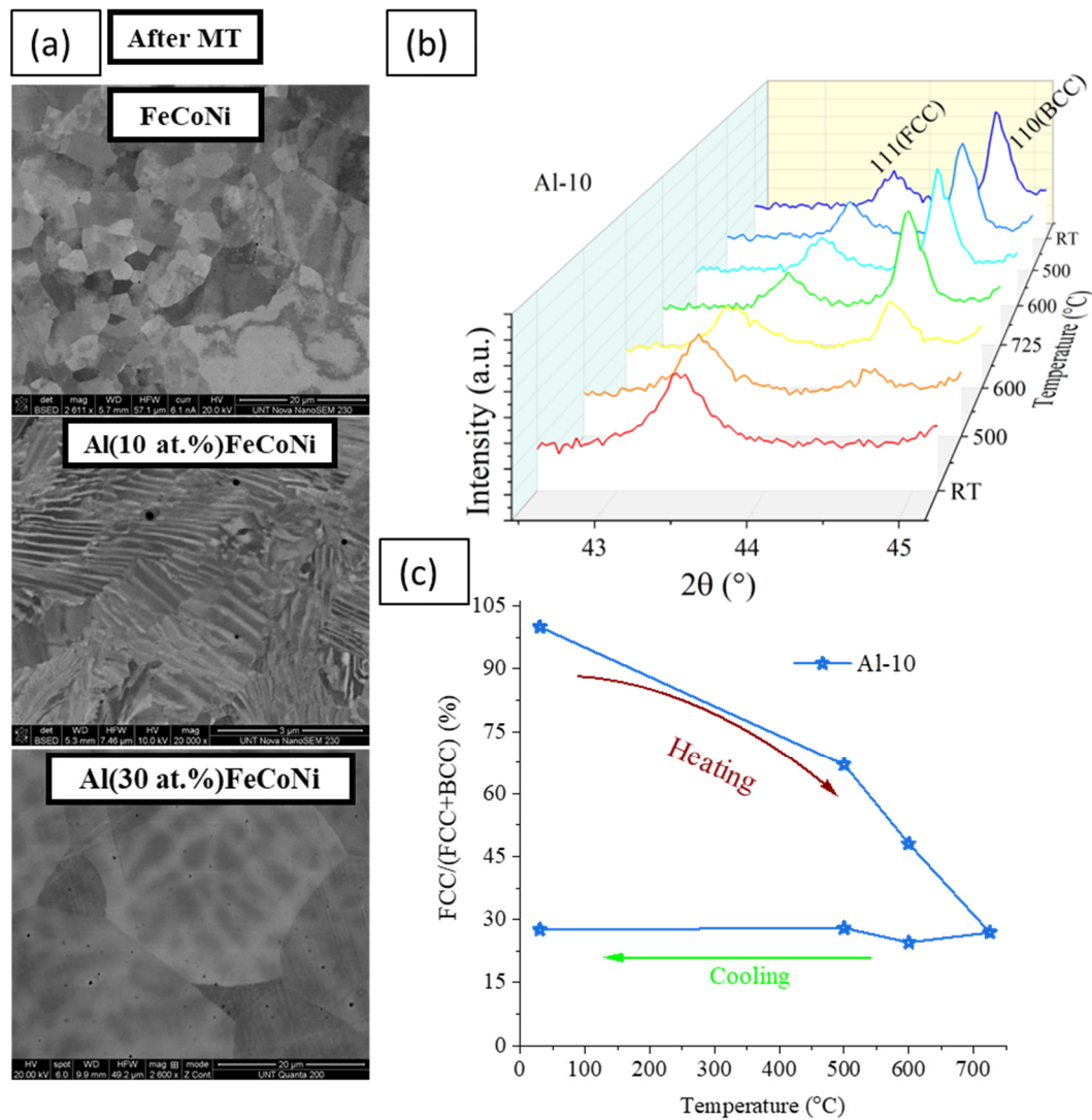
Figure 4. (a) Backscattered electron images of Al x (CoFeNi) CCA after MT measurements. (b) The in-situ high temperature XRD results for Al 10 (CoFeNi) CCA in the range from room temperature to 725 °C for both heating and cooling modes. (c) Variation in phase fraction as a function of temperature measured over heating and cooling cycles.
