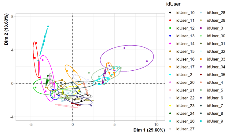
Fig. 2. Individuals factor map created using Factoshiny. One color per individual.
