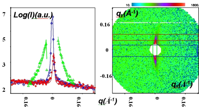
Figure 3. Modeling of the 2D neutron scattering produced by a 180 nm diameter AAO membrane filled with a 38 kDa protonated polymer (vertical membrane configuration). The left panel displays the experimental data along the areas defined by rectangles of the same color in the 2D pattern (right figure) and the fit by a simplified cylinder model (continuous lines). The green data correspond to the vertical direction, whereas blue and red data represent the two horizontal areas. Scattering conditions: D = 1.5 m; \lambda = 5.5 Å. Similar scattering is obtained without polymer or with other molecular weights.
