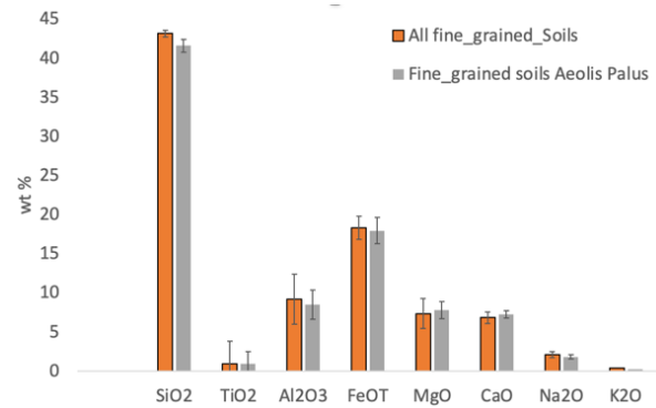
Fig. 3: Comparison of average composition obtained in fine-grained soils along the entire traverse (this study, in orange) and fine-grained soils from Aeolis Palus (in grey).
