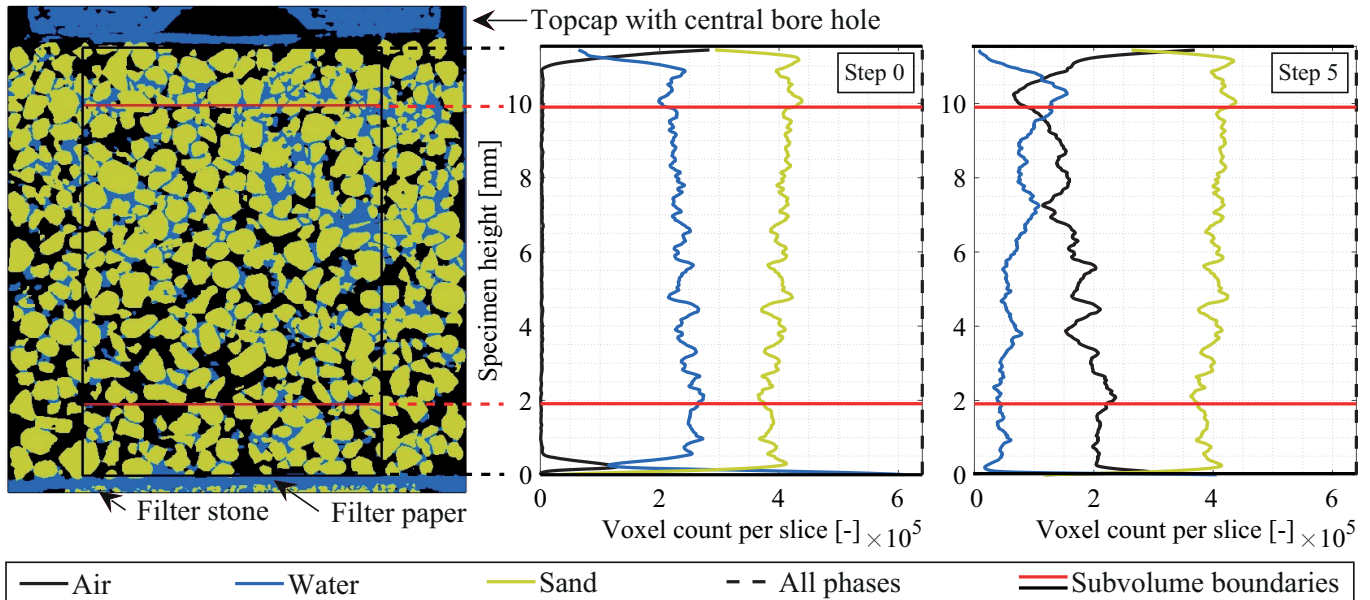
Figure 8. Location of subvolumes marked in a central vertical slice of segmented CT data for step 5 of the hydraulic experiment on Hamburg Sand and phase-specific voxel count for step 0 and step 5. Black boundary: Subvolume of 800 \text{ px} \times 800 \text{ px} \times 1145 \text{ px} . Red boundary: Subvolume of 800 \text{ px} \times 800 \text{ px} \times 800 \text{ px} .
