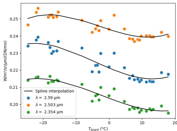
Figure 2: variation of the instrument response (ITF) with T_{\text{board}} for three sensitive wavelengths and their spline interpolation
