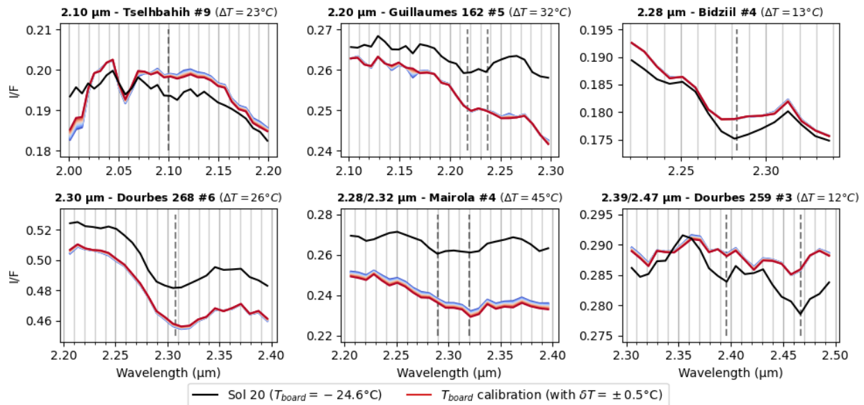
Figure 1: Sensitivity of various spectral signatures in the 2.0 – 2.5 \mu\text{m} range, the most sensitive to thermal effects, illustrated on the most representative observations. In each panel, the black line is the current flight calibration based on Sol 20 White SCCT observation, the color lines are the IR board temperature ( T_{\text{board}} ) calibration and the color gradient indicates its sensitivity at \pm 0.5^\circ\text{C} , corresponding to the T_{\text{board}} measurement precision. Dashed vertical lines highlight the detected absorption features. The temperature shift in parenthesis is the T_{\text{board}} difference between Sol 20 and the observation.
