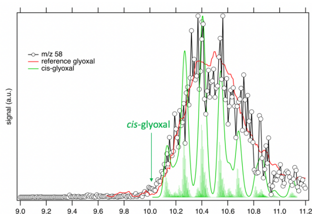
Figure 4. SPES of m/z 58 (open dots) compared to a simulated spectrum of cis -glyoxal (green line) and a reference threshold photoelectron spectrum of glyoxal (red line). The arrow indicates the calculated AIE of cis -glyoxal using the CCSD(T)/CBS limit method. The computed stick spectrum of cis -HPA is also displayed (green light sticks) and together with its respective simulated spectrum have been shifted by 80 meV from the calculated AIE.
