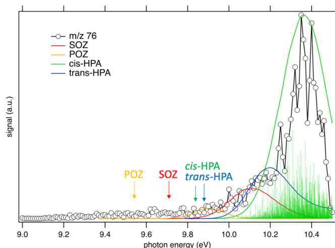
Figure 3. SPES of m/z 76 (open dots) compared to the simulated spectra of cis -HPA (green line), trans -HPA, SOZ, and POZ (orange line). Arrows indicate the calculated AIE of the C 2 H 4 O 3 isomers at the CCSD(T)/CBS level. The computed stick spectrum of cis -HPA is also displayed (green light sticks) and together with its respective simulated spectrum have been shifted by 80 meV from the calculated AIE. The stick spectrum of the other C 2 H 4 O 3 isomers is provided in Figure S2.
