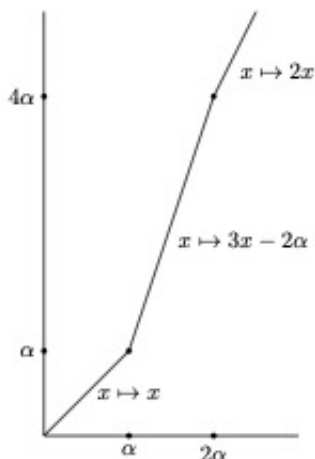
FIGURE 3. The homeomorphism g_\alpha .
