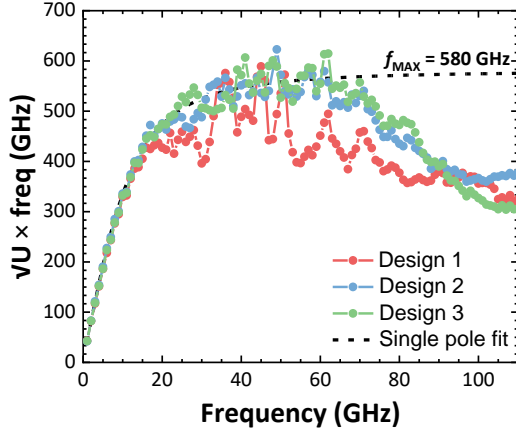
Fig. 10. Determination of f_{MAX} with gain-bandwidth product of a 0.4 \times 5 \mu\text{m}^2 DHBT at V_{CE} = 1.6 \text{ V} and J_C \approx 6 \text{ mA}/\mu\text{m}
