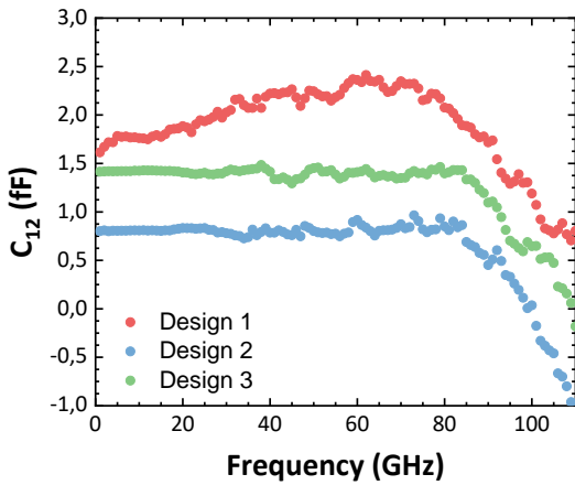
Fig. 8. Extracted port-1 to port-2 open capacitance C_{12} for the three test structure designs
