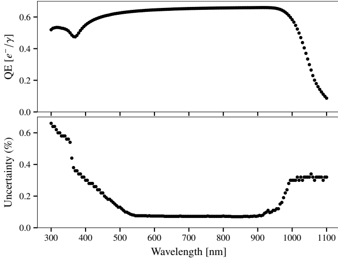
Fig. 6. Quantum efficiency of our reference Hamamatsu S2281 photodiode. Top : quantum-efficiency curve as measured by the NIST. Bottom : quoted relative uncertainty on the quantum uncertainty at the 95 % level ( 2\sigma ).
