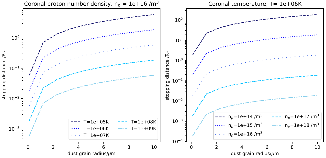
Figure 5. Stopping distance of dust grain as a function of grain size based on equation (15). In the left-hand panel, the number density is fixed at n_p = 10^{16} \text{ m}^{-3} and the coronal temperature varies. In the right-hand panel, the temperature is fixed at T = 1 \times 10^6 \text{ K} and the coronal number density varies. All other constants have the values in Table 2.
