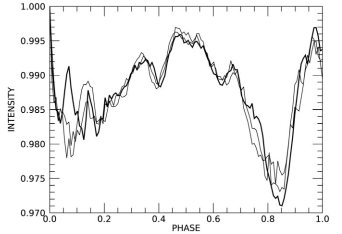
Figure 6. Model light curves for V374Peg created by filling a fraction of the stable points with dust particles of size 1 \mu m . Three different random samples of stable points are shown. The narrowest features have a width of about 0.05 in phase. The corresponding radial acceleration underestimates the distance of the cloud from the rotation axis by about 40 percent, as illustrated by the green arrow in Fig. 2.
