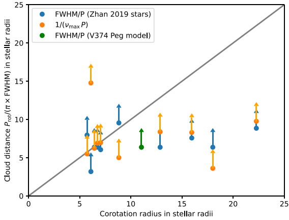
Figure 2. Lower limits on the radial distances r/R_* of the co-rotating clouds from the rotation axes of the 10 stars studied by (Zhan et al. 2019), versus Keplerian co-rotation radius. The blue points are measured using the full width at half maximum (FWHM) of the smallest dip feature in each light curve, while the orange points are derived from the highest-frequency clearly visible in the Fourier power spectrum of the light curve. The grey line of unit slope allows the cloud locations to be compared with the co-rotation radius. The green point, derived in the same way from the duration of the narrowest dip produced by clouds near the co-rotation radius in the synthetic light curve of V374 Peg (Fig. 6), illustrates the lower-limit nature of these measurements.
