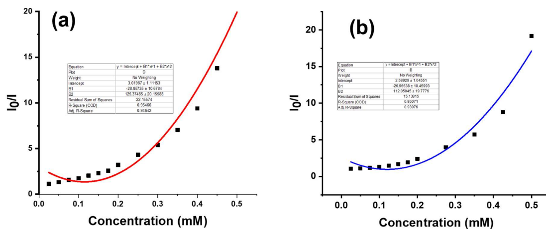
Figure. S24. Stern-Volmer plots for 7 at high concentration of (a) \text{Cr}^{3+} and (b) \text{Fe}^{3+}
