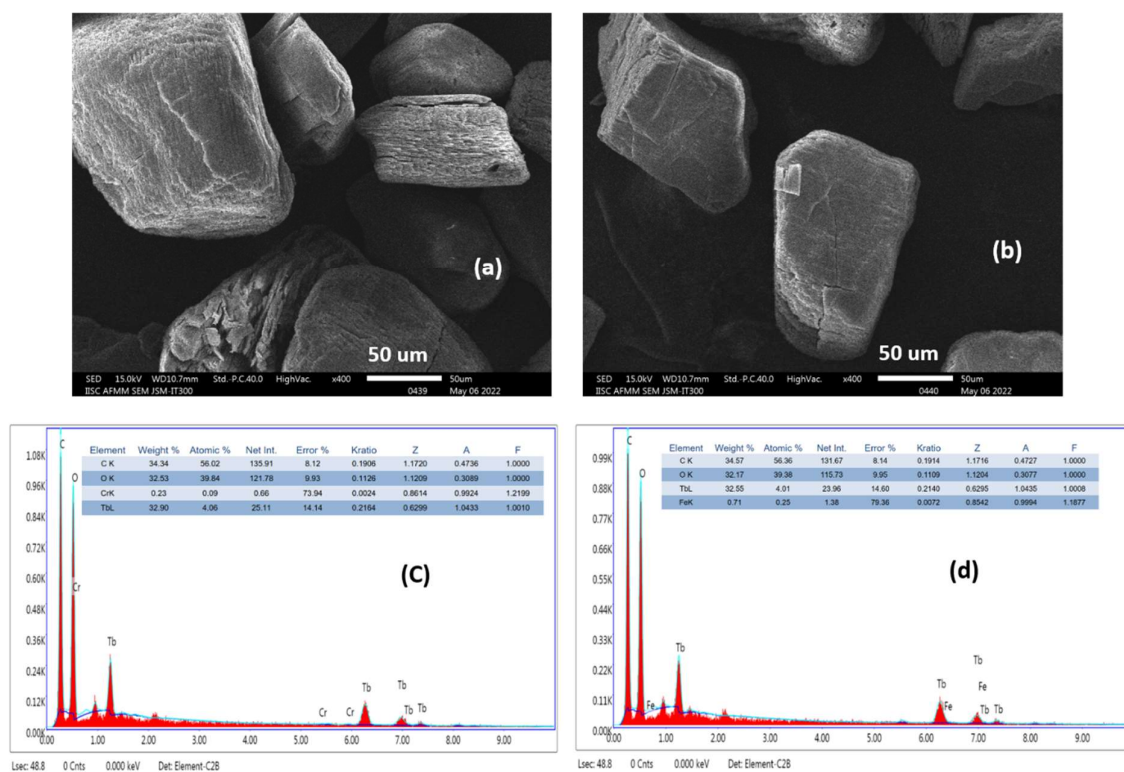
Figure S30: The SEM-EDX images after the sensing studies of \text{Cr}^{3+} (a and c) and \text{Fe}^{3+} (b and d) which indicated the structural integrity of compound 7
