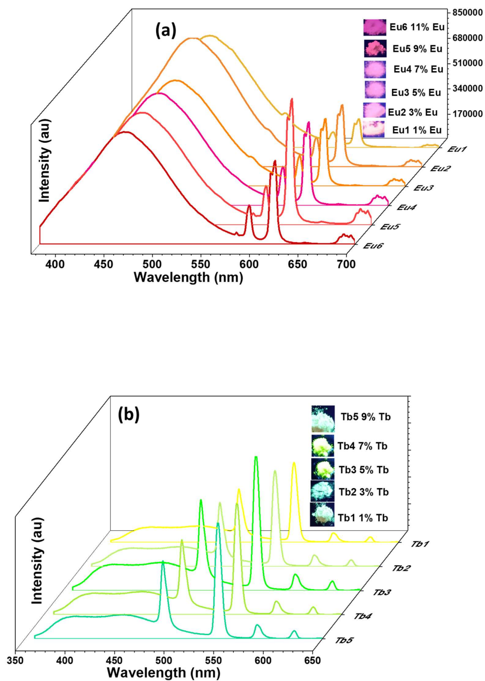
Figure S16: Different substitution of \text{Eu}^{3+} (a) and \text{Tb}^{3+} (b) in Y-MOF
