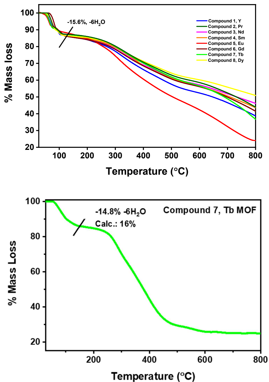
Figure S6. TGA plot of 2D compounds, Compounds 1 -8
