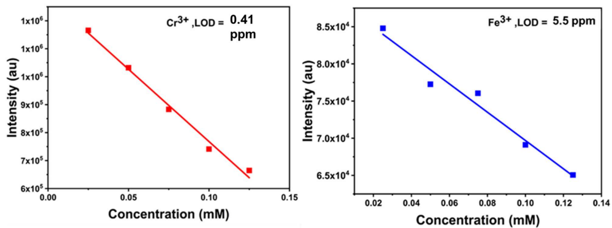
Figure S25: The LOD calculation graph for \text{Cr}^{3+} and \text{Fe}^{3+}
