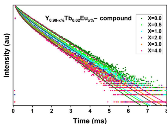
Figure 7: The decay curves for the luminescence of \text{Tb}^{3+} ions in \text{Y}_{0.98-x}\text{Tb}_{0.02}\text{Eu}_x\text{-} samples, with different \text{Eu}^{3+} concentrations (excited at 345 nm, monitored at 544 nm).
