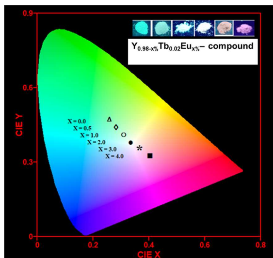
Figure 6: CIE color coordinate diagram of \text{Y}_{0.98-x}\text{Tb}_{0.02}\text{Eu}_x\text{-} samples with different \text{Eu}^{3+} concentrations ( 0 < x < 4.0 ). The insets are their corresponding digital photographs taken under 345 nm excitation.
