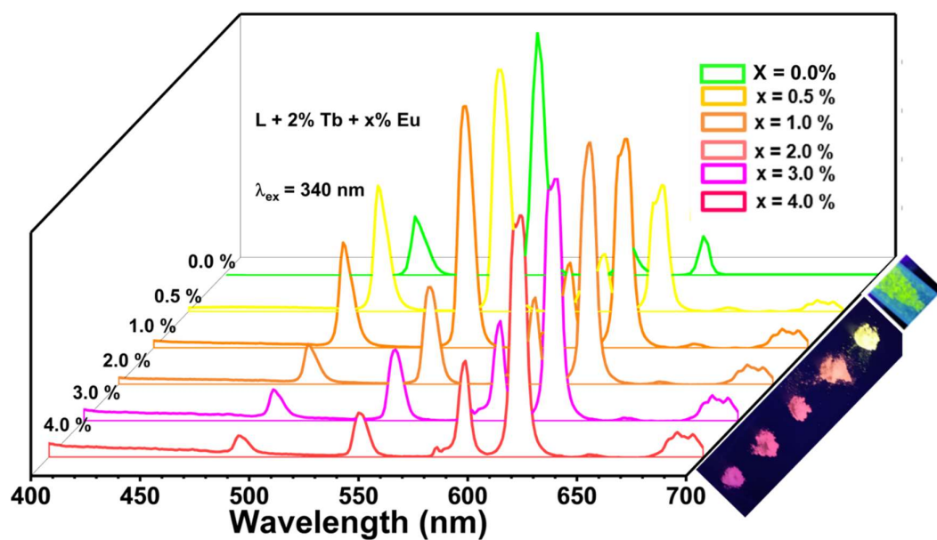
Figure S20: PL emission spectra ( \lambda_{\text{ex}} = 340 \text{ nm} ) of 2,5 BPTA + 2% Tb 3+ + x% Eu 3+ samples with different Eu 3+ concentrations ( 0 < x < 4.0 ).
