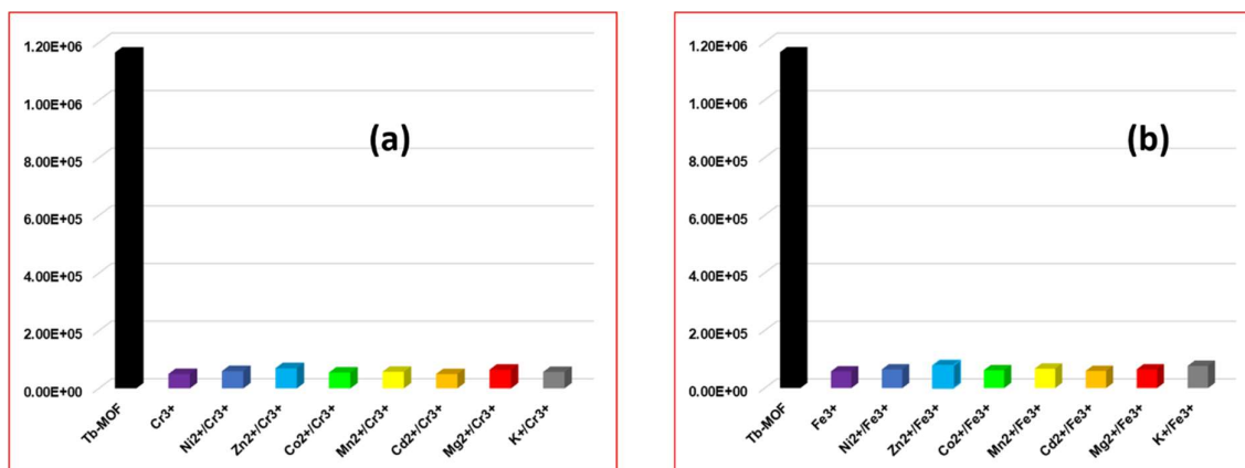
Figure S23. Comparison of the luminescence quenching effect of (a) Cr 3+ and (b) Fe 3+ ion Tb-MOF in presence of other competitive cations (5 x 10 -4 M).
