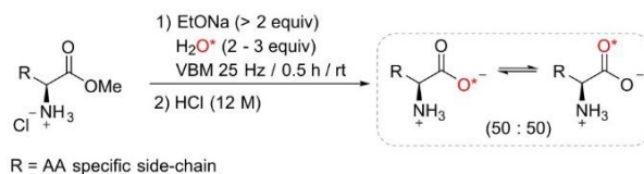
Scheme 1. Mechanochemical saponification procedure used to enrich free unprotected amino acids.
