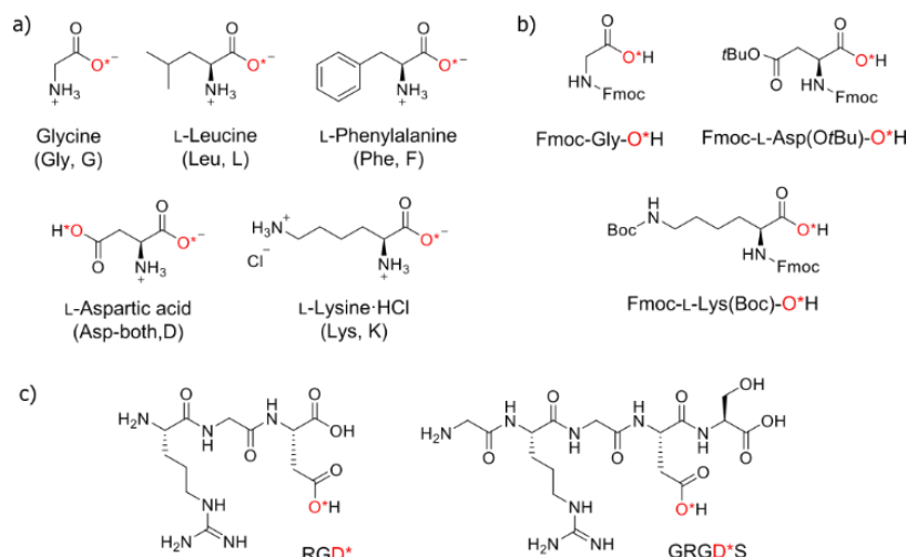
Figure 1. Scope of ^{17}\text{O} -labeled molecules prepared in this work: a) free amino acids, b) Fmoc/ t Bu-protected amino acids and c) peptides. Only one oxygen is labeled per carboxylic function using mechanochemistry, but globally, the label is distributed between both oxygen sites in the isolated phases (e.g. \text{C}=\text{O}^* and \text{C}-\text{O}^*\text{H} , 50 : 50), as evident from ^{17}\text{O} solid state NMR analyses.
