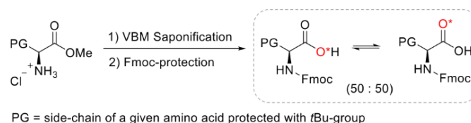
Scheme 3. Two-step procedure used for the synthesis of ^{17}\text{O}/^{18}\text{O} -enriched Fmoc/ t Bu-protected amino acids.
