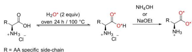
Scheme 2. Acid-catalyzed oxygen exchange procedure used for the enrichment of free amino acids. Both oxygen atoms per carboxylic function can become labeled by this procedure.
