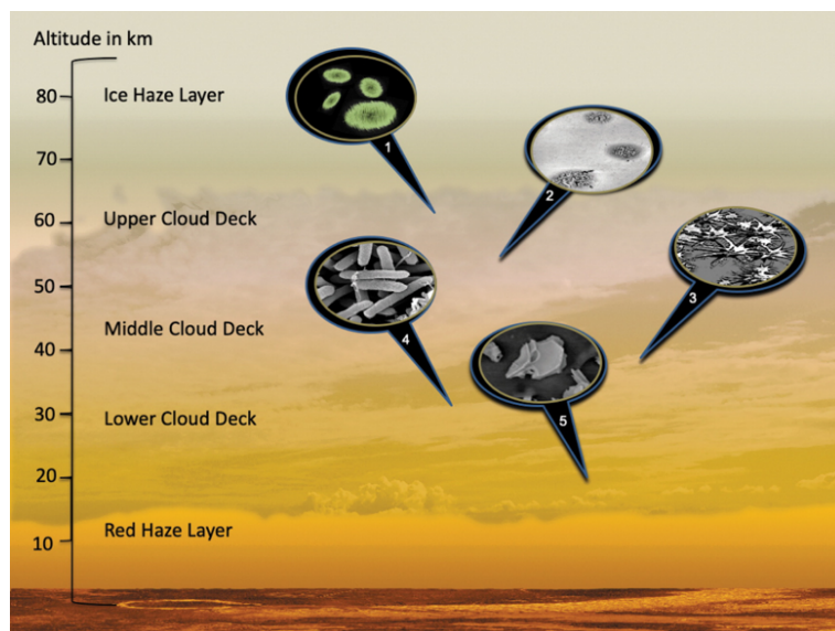
Fig. 10 Notional particles potentially to be encountered in the Venus cloud decks, inspired by terrestrial atmospheric sampling, to guide future instrument and analysis selection: (1) complex shapes with fluorescent properties, (2) particulate aggregates of sulfates and related compounds, (3) unidentified group of complex shapes adhered to an aerosol particle, (4) objects that resemble Earth bacteria or archaea, and (5) volcanic ash particles.
