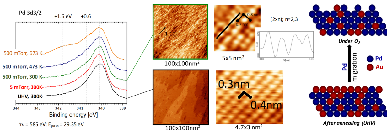
Figure 1. The PdAu(110) surface upon exposure to oxygen: (left) appearance of a high binding energy shoulder on Pd 3d 3/2 XPS peak with increasing oxygen pressure and temperature; (center) reconstruction of the surface as seen by STM and Pd segregates to the surface; (right) schematics of the evolution.
