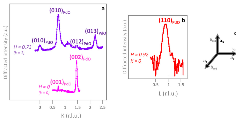
Figure 3. PdO peaks measured by SXR D along several directions of the reciprocal space (along K in with L=0 and H=0 and H=0.73 , in a ; along L with H=0.92 and K=0 , in b ) in the frame of the fcc PdAu(110) surface by (a_1, a_2, a_3) with the Miller indices (H, K, L) and the oxide peaks are labeled with the Miller indices (h, k, l) in the PdO frame (a_{\text{oxi}}, b_{\text{oxi}}, c_{\text{oxi}}) defined in c .
