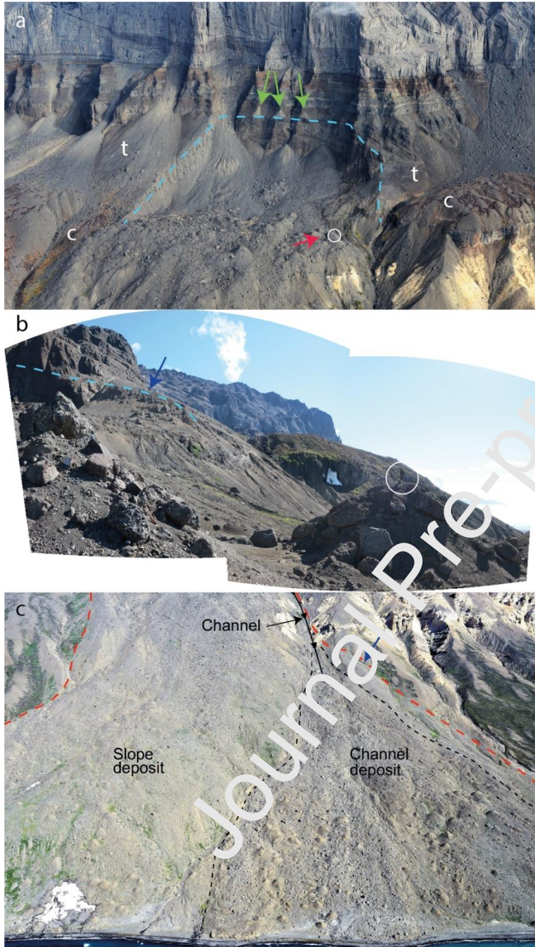
Figure 2. [1.5 column, text to the right] Field photographs from 2019 a) Oblique aerial photo of the source area in the talus slope below the grey/brown cliff of Paleocene hyaloclastite and above the light-yellow Cretaceous sediments. Talus and colluvium on the surrounding slope are showed with t and c respectively. The stippled blue line outlines the backscarp and the green arrows shows the top of the relict talus slope, the lower part of which was involved in the landslide. The red arrow shows the position and direction of the photo in Fig. 2b and the white circle highlights the molard with the person on top in Fig. 2b. b) mosaic of two
