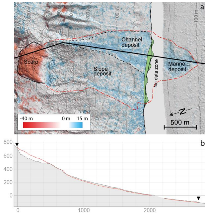
Figure 6 [1½ column] a) DEM of Difference (DoD) of the Niiortuut landslide made from 1949 and 1953 DEM's from the onshore area and the recent bathymetrical mapping for the offshore area. The green polygon on the shore shows how much the coastline advanced during the landslide as observed in the 1953 aerial images. The hillshade overlay is from the 1953 DEM. b) Elevation profile through the scarp and the channel deposit of the landslide (along bold black line in a). The red line is the 1949 pre-landslide elevation and the dark grey with light grey filling is the 1953 post landslide elevation.
