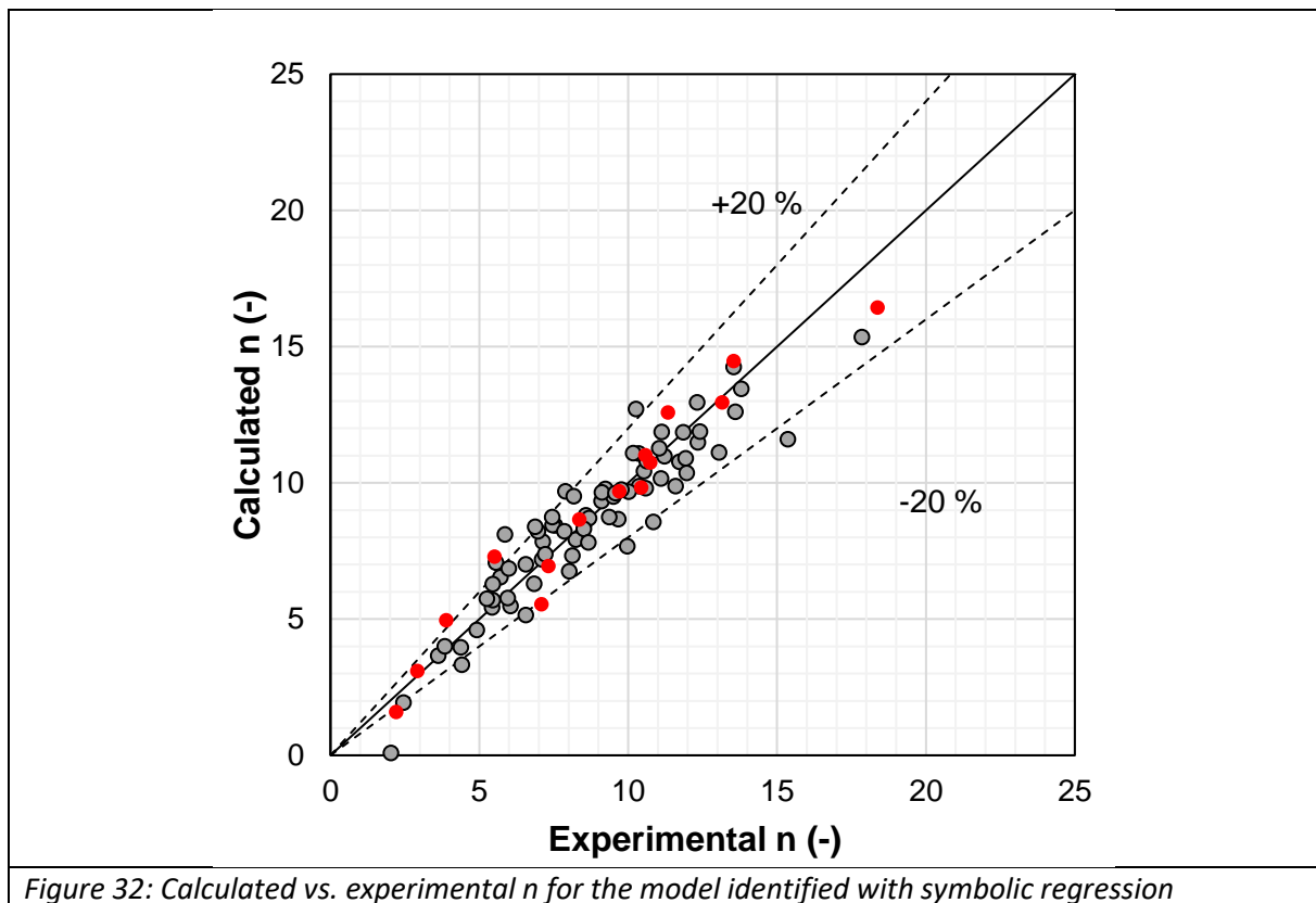
Figure 32: Calculated vs. experimental n for the model identified with symbolic regression
