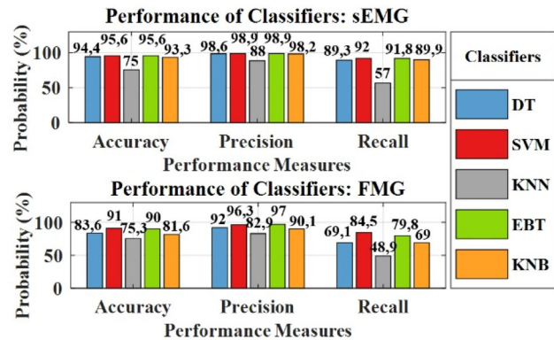
Figure 2. Performance of classifiers.
