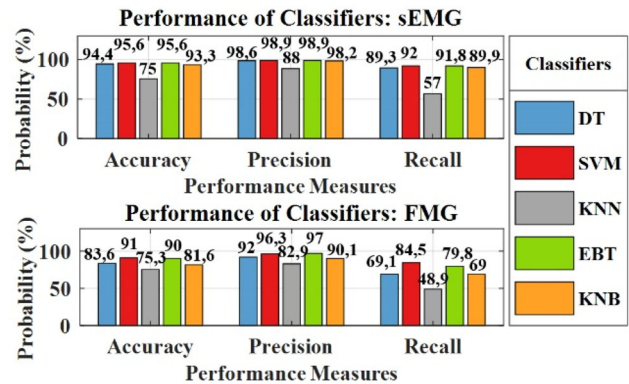
Figure 2. Performance of classifiers.
