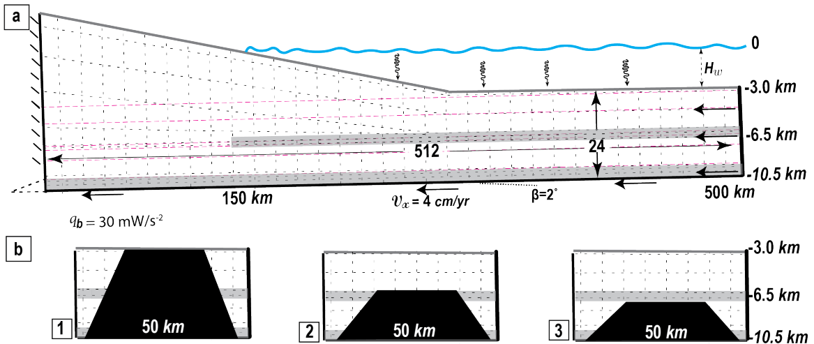
Figure 3: a. Model set-up. Boundary conditions are a non-deformable backstop on the left side, a constant velocity in the x-direction of 4\text{ cm}\cdot\text{year}^{-1} , free surface or water pressure considered below sea level and basal heat flow calibrated from BSR. b. Three different initial seamount geometries.
