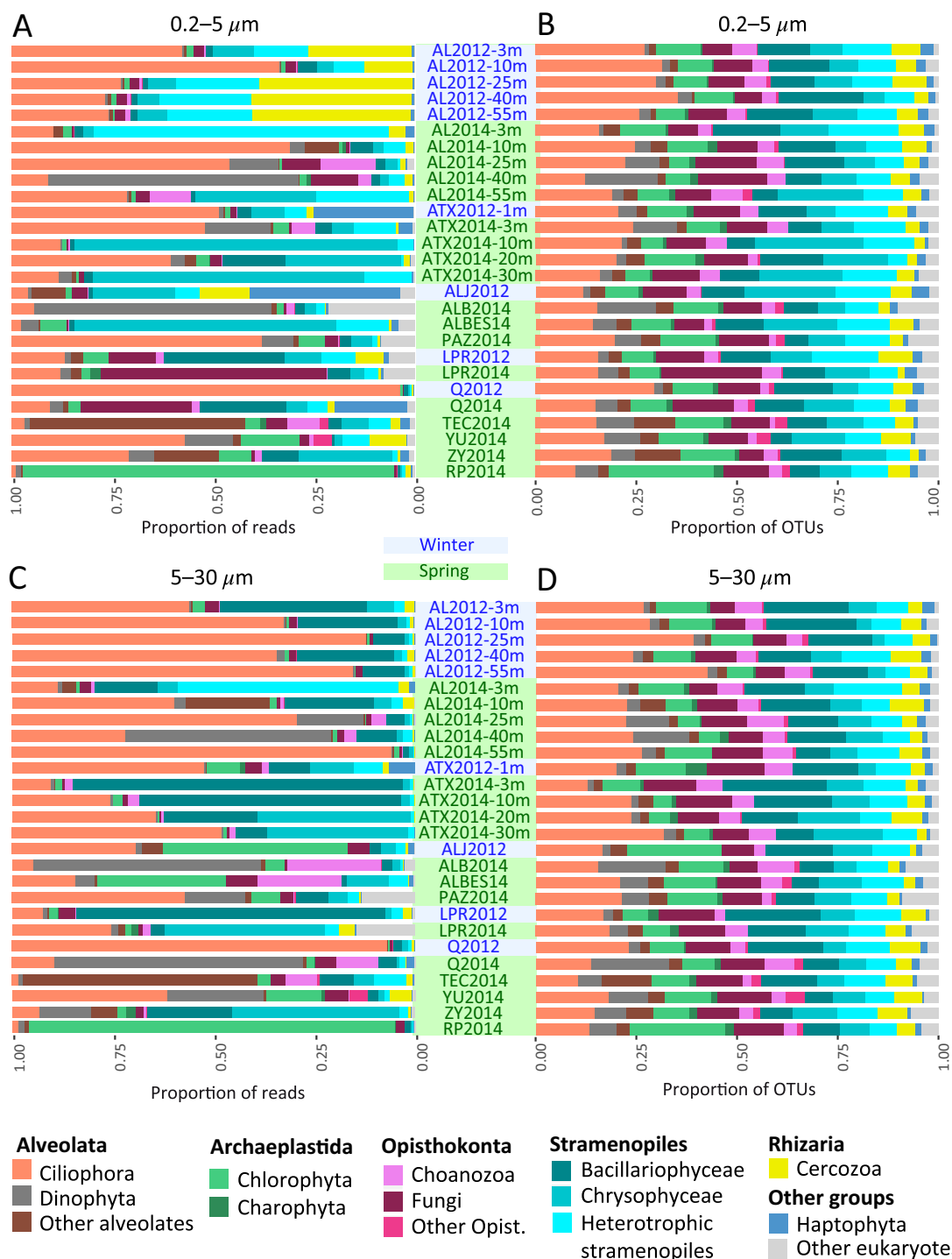
Fig. 3. Histograms showing the phylogenetic diversity and relative proportion of 18S rRNA genes amplified from planktonic samples collected from Mexican lakes. (A) Relative abundance of eukaryotic sequences from the 0.2–5- \mu\text{m} cell fraction. (B) Diversity shown as relative abundance of OTUs in the 0.2–5- \mu\text{m} fraction. (C) Relative abundance of eukaryotic sequences from the 5–30- \mu\text{m} cell fraction. (D) Diversity shown as relative abundance of OTUs in the 5–30- \mu\text{m} fraction. Detailed histograms of the category “other eukaryotes” are provided in Supplementary Fig. S4.
