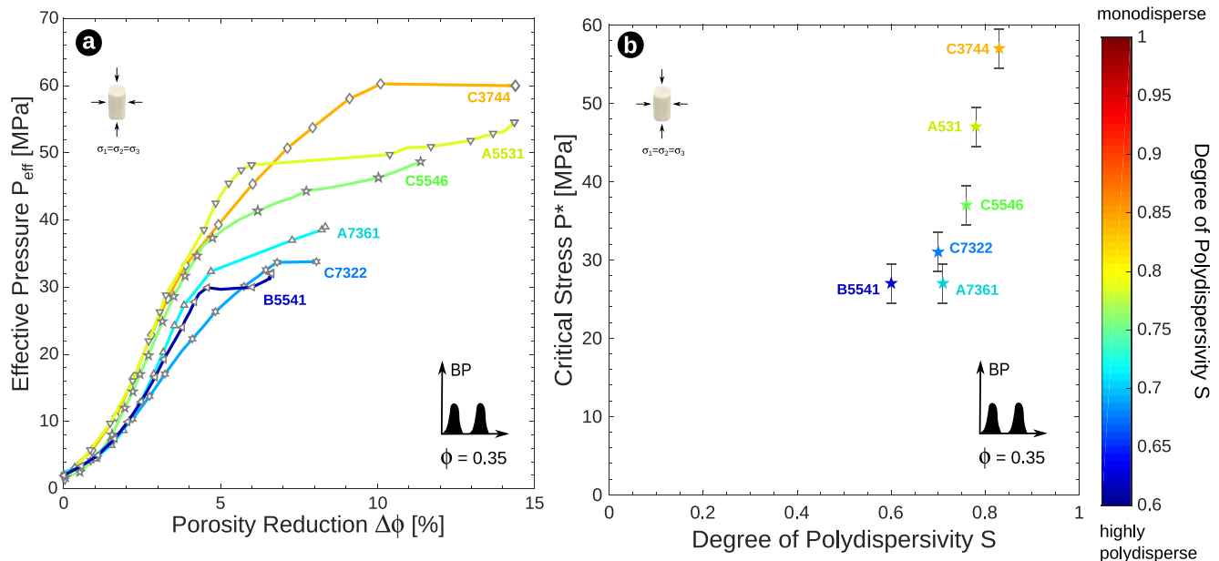
Figure 6. Mechanical data for the hydrostatic compression of bidisperse synthetic samples with a porosity of 0.35. (a) The hydrostatic curves are shown as the effective pressure against the porosity reduction, using a colormap for the degree of grain size distribution polydispersity. The name of the grain size distribution of each sample is indicated at the end of the corresponding hydrostat and corresponds to both Table 1 and Figure 2. (b) The critical stresses for the onset of grain crushing ( P^* ) are plotted against polydispersity.
