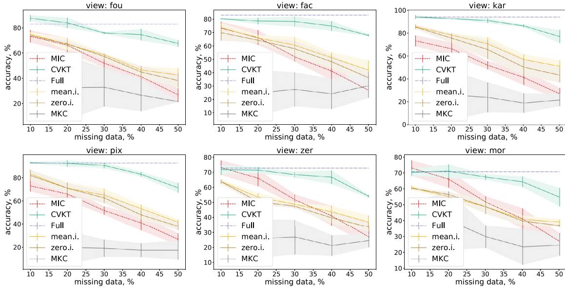
Fig. 6. Accuracies of classification with full, mean inputed, zero inputed, CVKT-completed and MKC-completed kernel matrices for all six views of the digits dataset as a function of level of missing data in views. The MIC results are for a common representation, and thus identical in all the plots.
