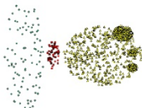
(MinPts=4, Eps=9.92)
