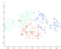
K-means (3 Clusters)
