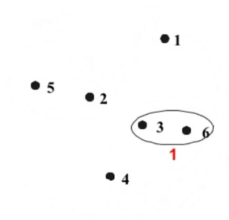
Nested Clusters
