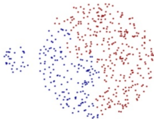
Two Clusters
