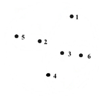
Nested Clusters
