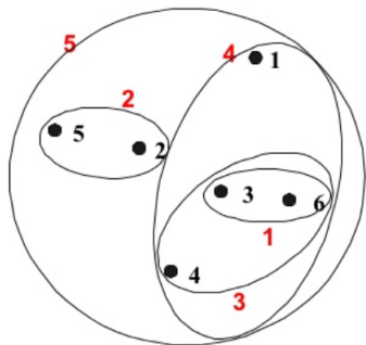
Nested Clusters
