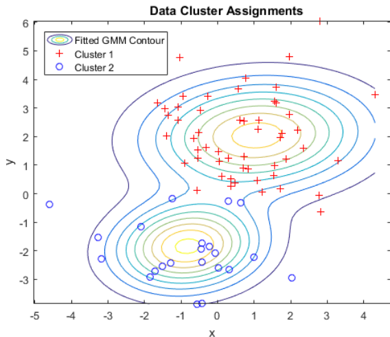
Figure: Example of 2 clusters with Gaussian distributions
