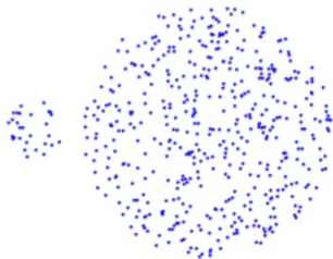
Original Points
