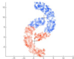
K-means (2 Clusters)
