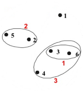
Nested Clusters
