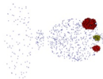
(MinPts=4, Eps=9.75)
