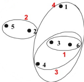
Nested Clusters
