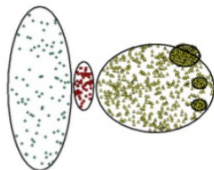
Original Points
