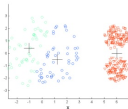
K-means (3 Clusters)
