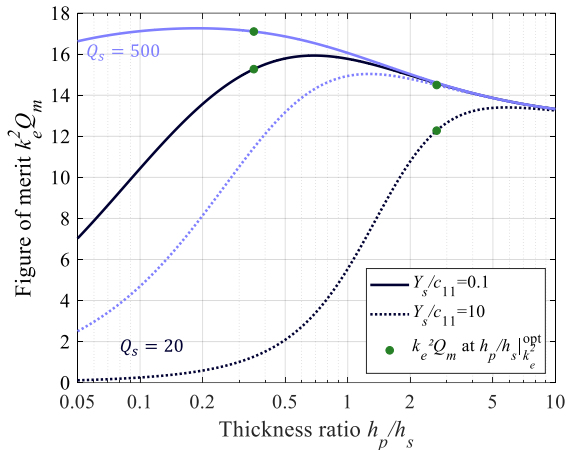
Figure 9: Theoretical value of k_e^2 Q_m considering \mathcal{R}_L = 1 , for k_{e31}^2 = 0.18 , Q_p = 100 and Q_s \in \{20; 500\} .
