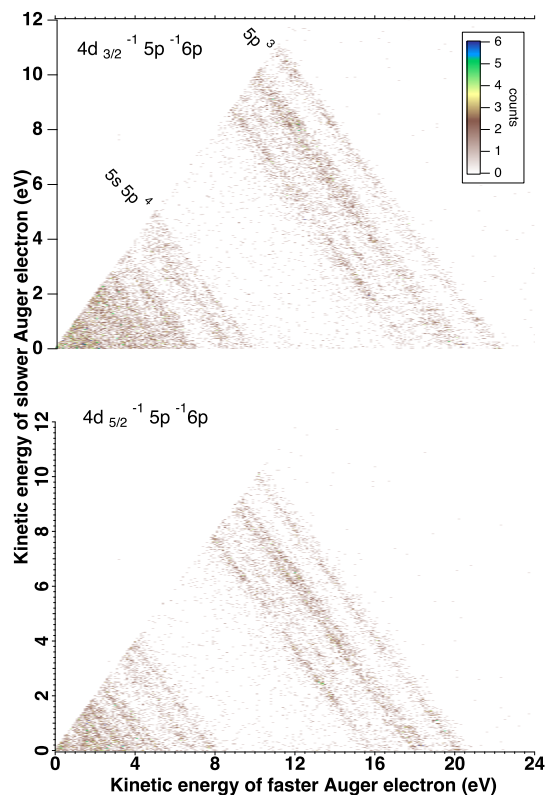
Fig. 6 Decay of xenon 4d 5p^{-1} 6p shake states by emission of two Auger electrons. The three electrons are detected in coincidence with \text{Xe}^{+3} ion. The 2D plot of the Auger double electrons are filtered according to the satellite photoelectron lines \sim 49 eV (top) and \sim 51 eV (bottom).
