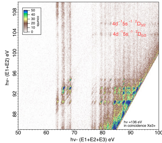
Fig. 9 2D map of core valence double photoionization of Xe atoms at 136 eV photon energy presenting the energy of the double ionized states h\nu - (E_1 + E_2) against the energy of the final \text{Xe}^{3+} states h\nu - (E_1 + E_2 + E_3)
