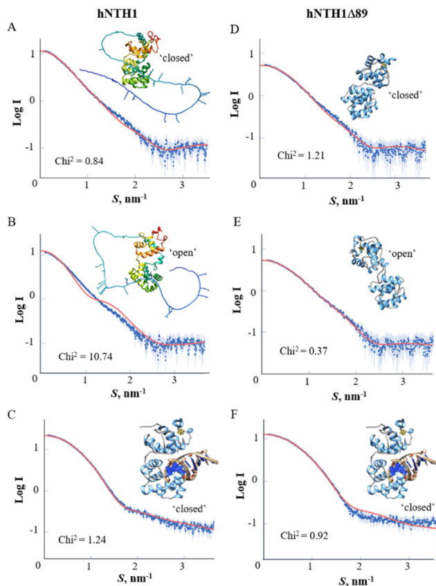
Fig. 2 Conformational flexibility of hNTH1 and hNTH1 \Delta 89 in solution. Crystol derived fits of the experimental SAXS scattering curves (blue) to the theoretical scattering curves (red). (A–C) hNTH1 vs. AlphaFold derived model of (A) ‘closed’ and (B) ‘open’ state hNTH1, (C) hNTH1 bound to DNA vs. ‘closed’ model of hNTH1 \Delta 63 (PDB, 7RDS) bound to dsDNA (extracted from PDB 1P59). (D–F) hNTH1 \Delta 89 vs. (D) ‘open’ and (E) ‘closed’ state of hNTH1 \Delta 63; and (F) hNTH1 \Delta 89 bound to DNA vs. ‘closed’ state of hNTH1 \Delta 63 bound to dsDNA. \chi^2 values (goodness of fit) are indicated. The respective atomic models used for the fits are illustrated in rainbow from N- to C-terminus for the AlphaFold models and in blue (protein) and beige (DNA) models of hNTH1 \Delta 63. Positively charged residues (Arg and Lys) located in the flexible NTD are shown as sticks in (A) and (B).
