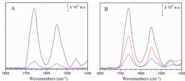
Fig. 1 SEIRA spectra of hNTH1 and hNTH1 \Delta 89. (A) hNTH1 and (B) hNTH1 \Delta 89 adsorbed on a gold electrode surface coated with MUA (black), damaged DNA (red) and undamaged DNA (blue) SAMs.
