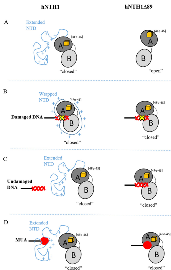
Fig. 3 Schematic representation of orientations and conformations of hNTH1 (left) and hNTH1 \Delta 89 (right). (A) Models of hNTH1 and hNTH1 \Delta 89 in DNA free states, based on the fitting of SAXS data to experimentally derived and predicted structures. (B) Damaged-DNA terminated SAMs: both hNTH1 and hNTH1 \Delta 89 adopt a ‘closed’ conformation and the NTD of hNTH1 wraps tightly around the protein/DNA. (C) Undamaged-DNA terminated SAMs: only hNTH1 \Delta 89 binds to the SAM, most likely in a ‘closed’ conformation. (D) MUA-terminated SAMs: hNTH1 and hNTH1 \Delta 89 bind to the SAM in different orientations, suggesting that the NTD bearing positively charged residues plays a role in binding to negatively charged MUA.
