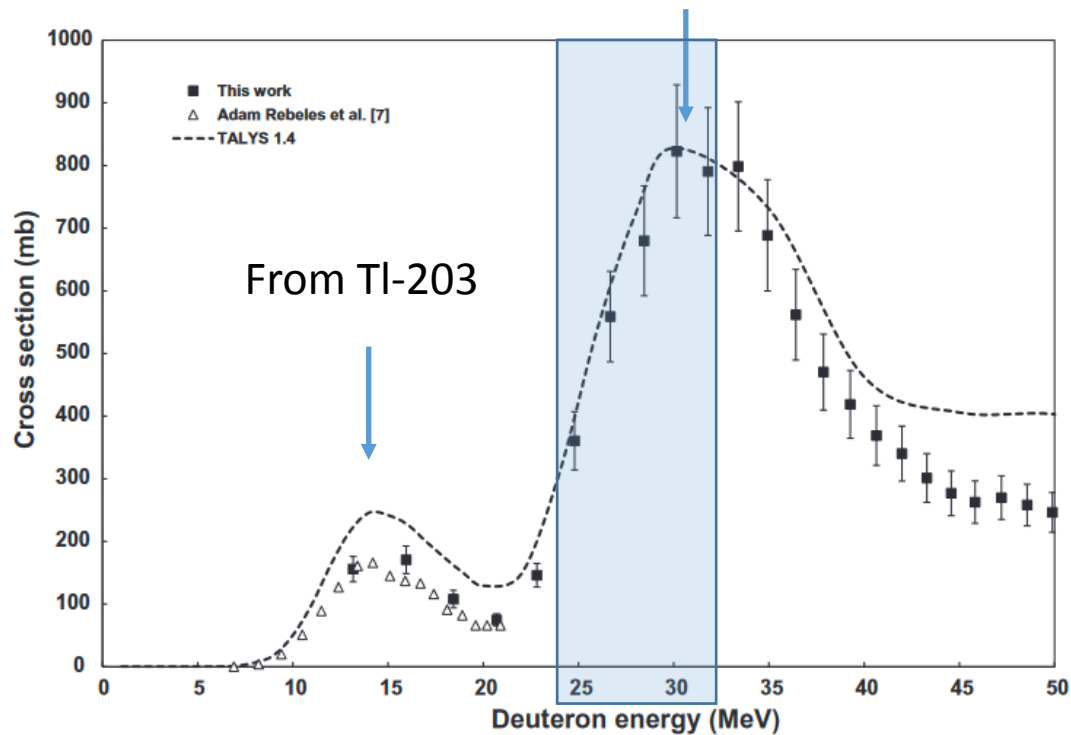
Excitation function for the ^{nat}\text{Tl}(d,xn)^{203m2+m1+g}\text{pb} reaction.
