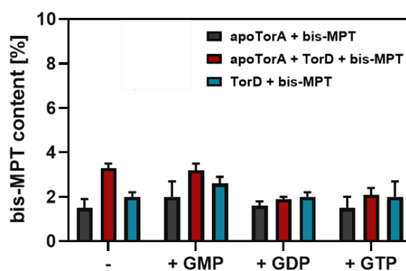
Figure 4. Effect of the presence of TorD and effect of free nucleotides in the reconstitution mixture on the insertion of bis-Mo-MPT into apo-TorA. Here, 1.3 \mu\text{M} apo-TorA, 2 \mu\text{M} TorD or both were incubated with bis-Mo-MPT isolated from 30 \mu\text{M} YdhV, and 50 mM GMP, GDP or GTP was added prior to the reconstitution mixture. Bis-Mo-MPT was detected in form of its fluorescent oxidation product dephospho-FormA.
